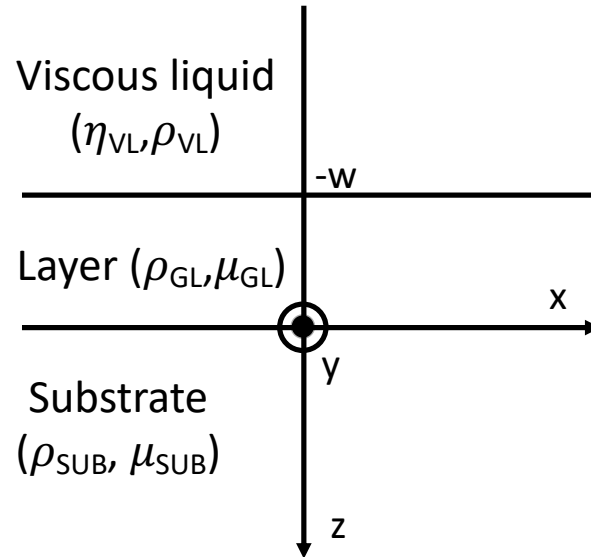
Figure 1. Scheme of the Love-wave structure with the 3 stacks [17].
