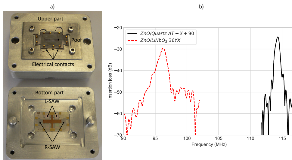
Figure 3. Microfluidic cell and ZnO/Quartz AT – X + 90 structure (a); insertion loss of the transmission response (S21) observed with fluid (water) interaction for both L-SAW devices (b).
