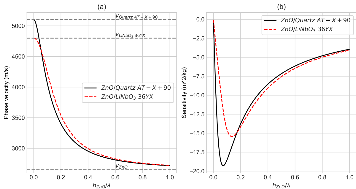
Figure 2. Theoretical calculated phase velocity (a) and mass sensitivity (b) for the first Love mode as a function of normalized guiding-layer thickness.
