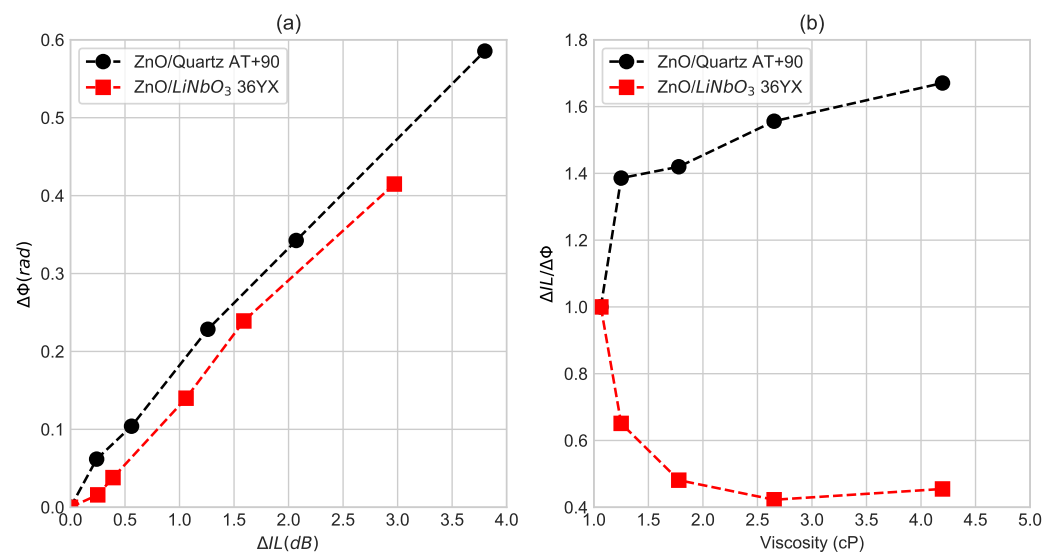
Figure 4. Experimental phase shift vs. insertion loss for different fluid viscosity (a) and relative acoustic ratio as a function of the viscosity (b) for both structures.
