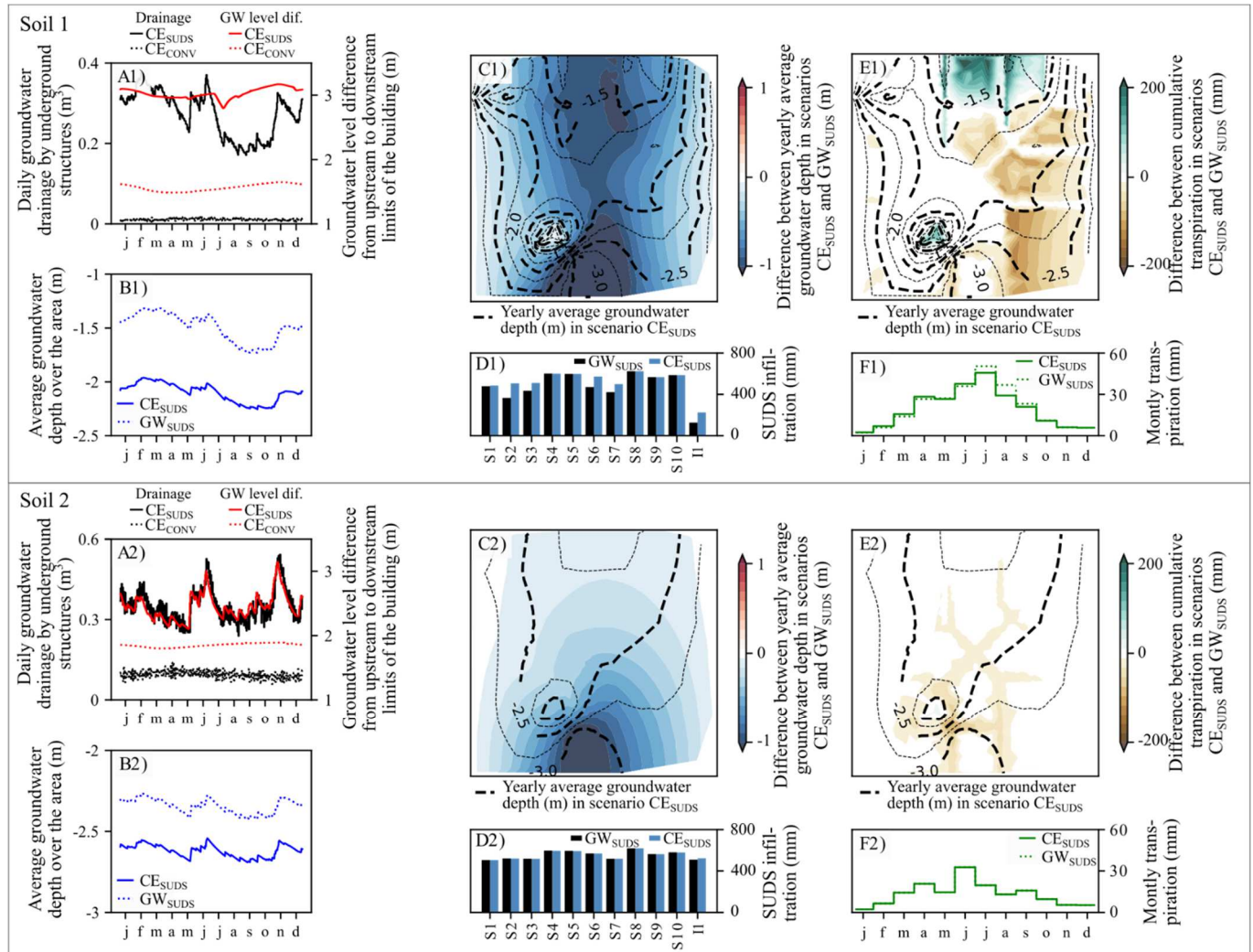
Figure 8 : Simulation results for the scenario CE_{SUDS} (cumulative effect of all underground structures) for soil 1 (sandy loam) and 2 (sand). Comparison with scenario CE_{CONV} (corresponding scenario without SUDS) to assess the SUDS influence on daily groundwater volumes drained by underground structures and on groundwater level difference between upstream and downstream limits of impervious foundations (A). Comparison with scenario GW_{SUDS} (no underground structure) to assess the cumulative effect of underground structures on average groundwater depth over the domain (B), on yearly average groundwater depth at each point of the domain (C), on infiltration within SUDS (D), on cumulative transpiration at each point of the domain (E) and on monthly transpiration over the domain (F).
