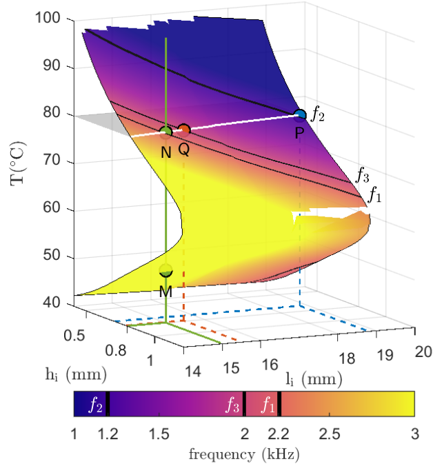
Figure 4: Surface gathering all the configurations of length l_i and thickness h_i leading to a perfect absorption at operating temperature T . The absorption frequency is represented by the colormap. The points M and N are the two critical coupling configurations for a nominal geometry occurring at 51°C and 80°C. The white line represents a chosen temperature of 80°C and the black lines are the isolines of the target frequencies f_1 , f_2 and f_3 . The points M, P and Q denote the configurations from the temperature and frequency set point which corresponds to the intersection between the white and black lines.
