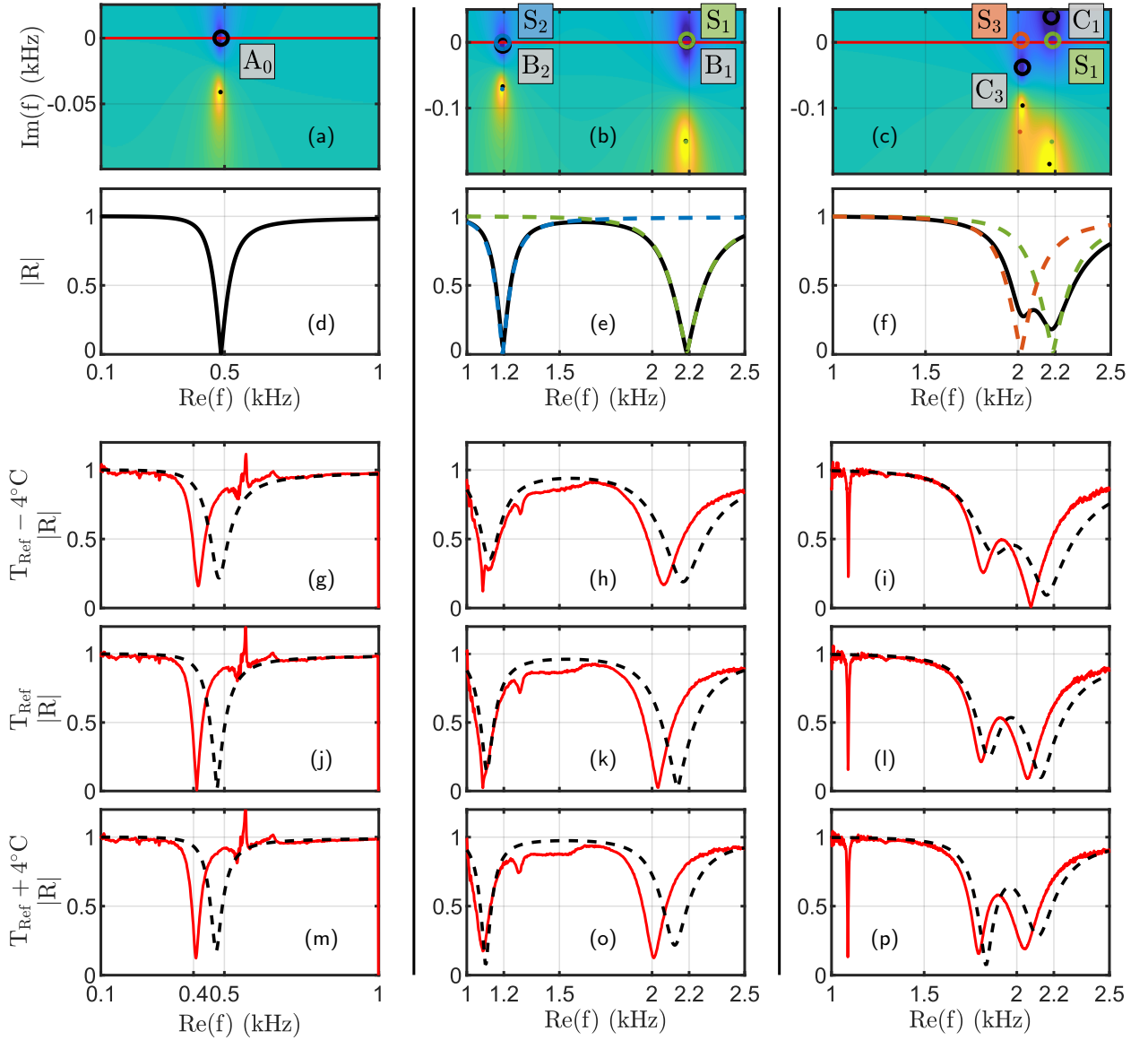
Figure 5: (a) \log|R| in the complex frequency plane of the single-blade (A) at 85°C. The zero and pole are marked by the black circle and dot. The label A_0 names the zero induced by the blade 0 of the system (A). (d) |R| along the real frequency axis of the single-blade (A). (b) \log|R| in the complex frequency plane of the dual-blade (B) at 80°C. The labels B_1 and B_2 denote the zeros induced by the blades 1 and 2 of the system (B). The color labels S_1 and S_2 , marked with color circles, denote the position of the zero induced by the blade 1 and 2 of a two single-blades. (e) |R| along the real frequency axis of the double-blade (B) in black. The dashed color lines correspond to |R| of the compared single-blades. (c) and (f) same as (b) and (e) for the dual-blade (C) involving the blades 1 and 3. (g) to (p) present the measured |R| in red solid lines of the systems (A) (first column: (g), (j) and (m)), (B) (second column: (h), (k) and (o)) and (C) (third column: (i), (l) and (p)), compared to the numerical |R| in black dashed lines computed accounting for the machining geometry. In lines (i.e., (j), (k) and (l)) are the resulted |R| for different operating temperature around T_{\text{Ref}} , see Tab. 2.
