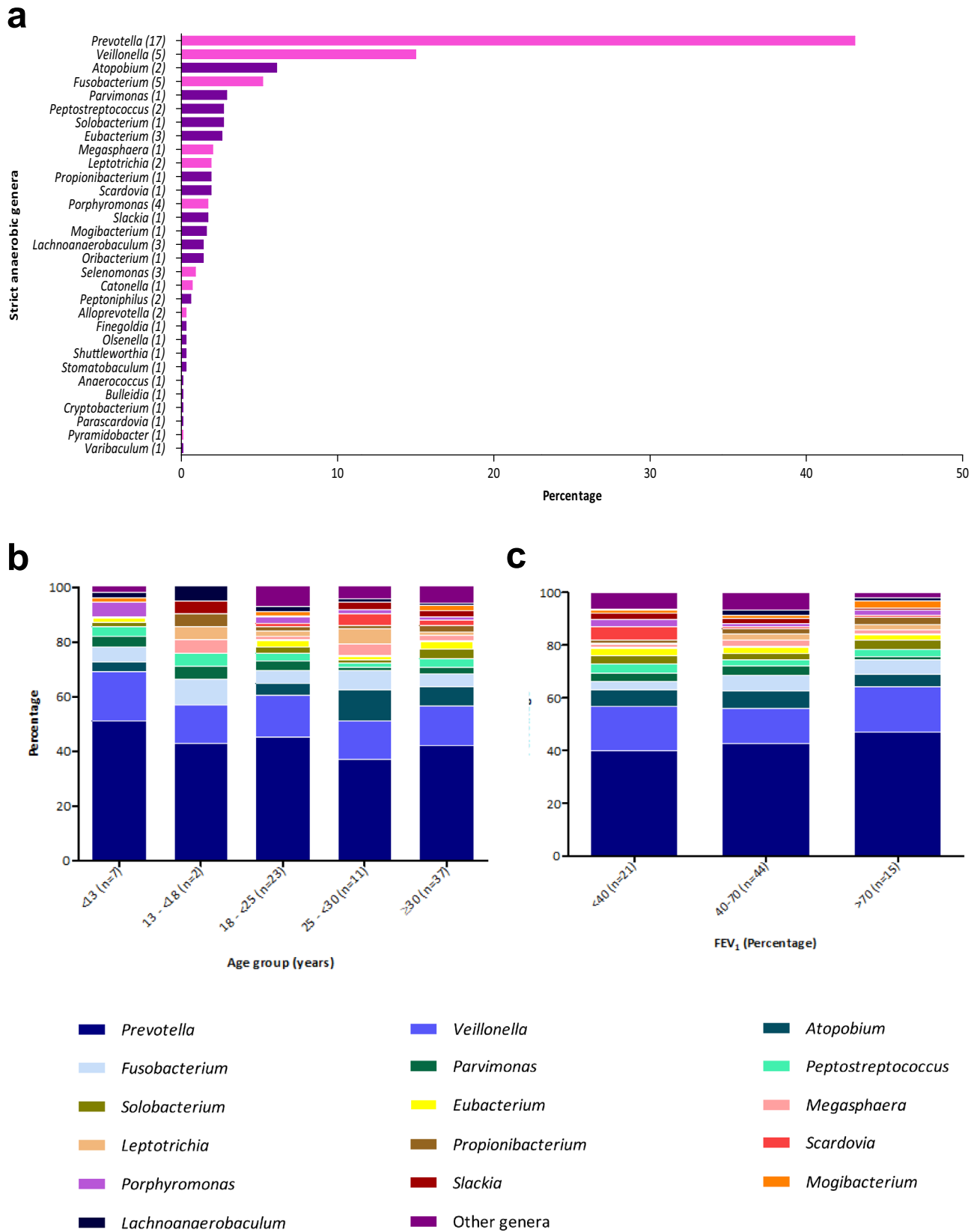
Figure 2. Extended-culture approach results. (a) Description of strict anaerobic genera identified in 112 sputum samples: Gram-positive genera are shown in purple, Gram-negative genera in pink, and number of species in brackets. (b) Prevalence of strict anaerobic genera identified according to patient age group (80 patients). (c) Prevalence of strict anaerobic genera identified according to patient lung function evaluated by Forced Expiratory Volume in one second (FEV 1 ) (80 patients).
