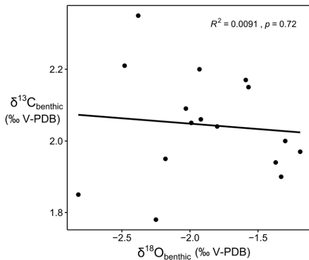
Fig. 5. \delta^{13}\text{C} vs \delta^{18}\text{O} cross plot of the isotope ratio measurements of the benthic foraminifera, showing no statistically significant correlation.
