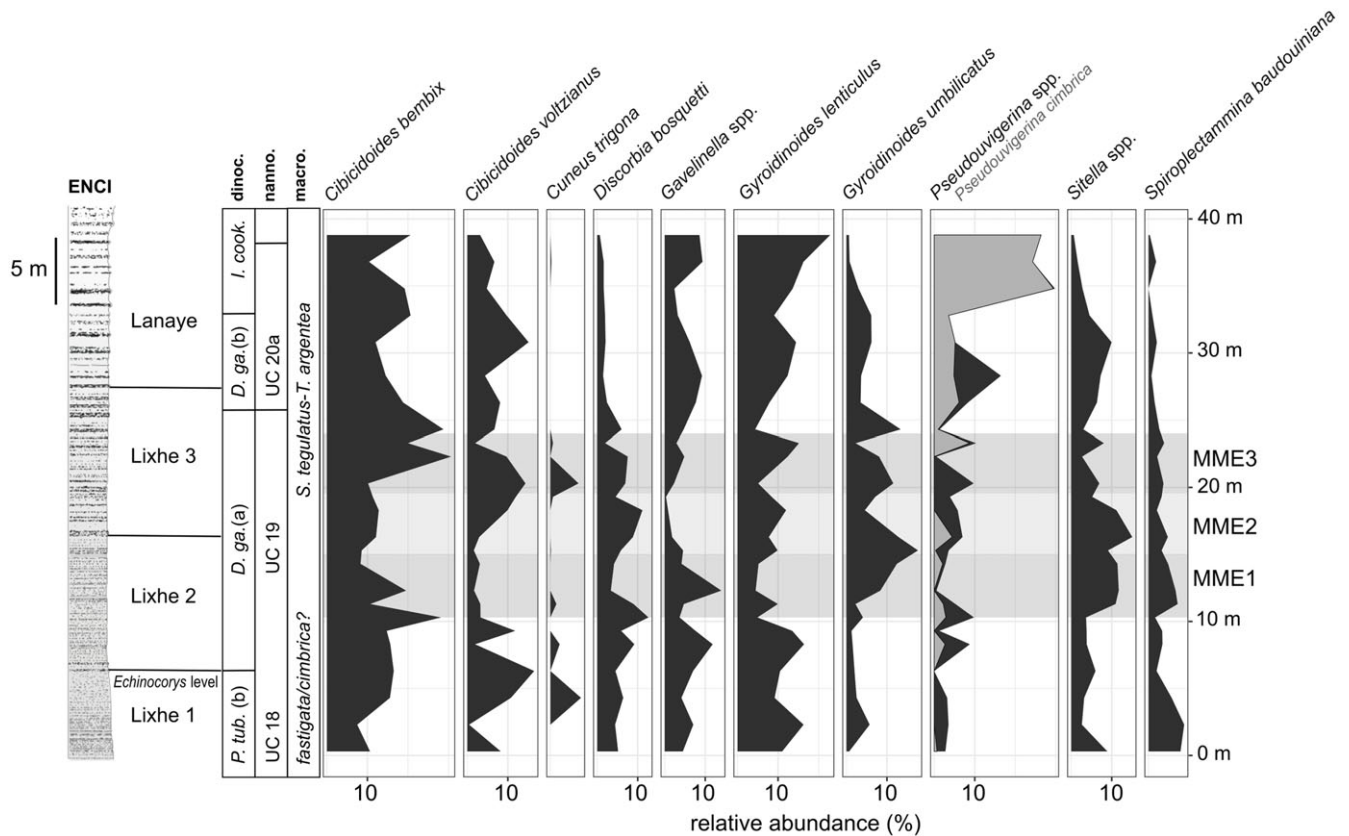
Fig. 8. Relative abundances of the most common benthic foraminifera taxa and Cuneus trigona at the ENCI quarry. Biostratigraphy after Vellekoop et al. (2022), for abbreviations see caption of Fig. 6.
