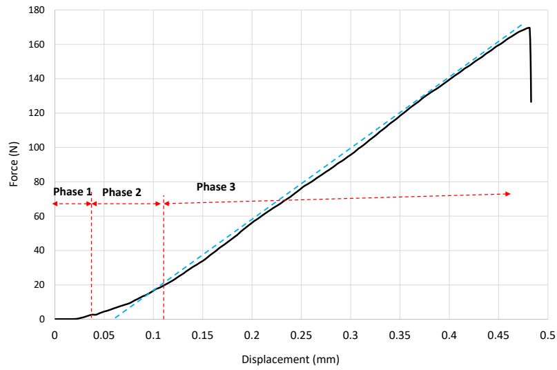
Fig. 2. Example of load-displacement curve of a specimen with a span length of L=150\text{mm} .
