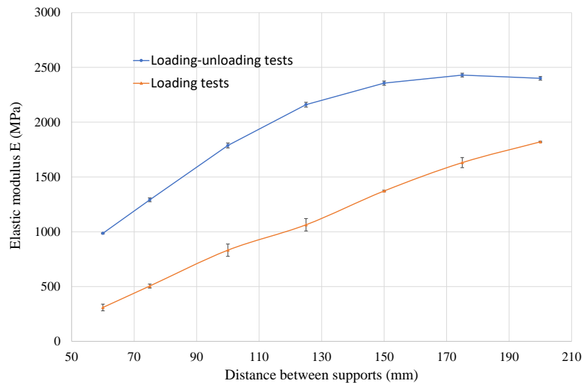
Fig. 8. Elastic modulus evolution as function of span length.
