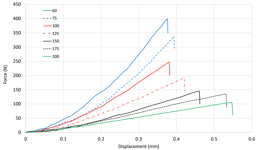
Fig. 5. Load-displacement curves of the printed specimen at different distance between supports.
