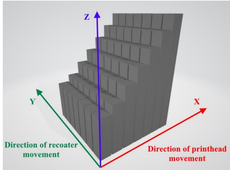
Fig. 1. Printing configuration of the specimens
