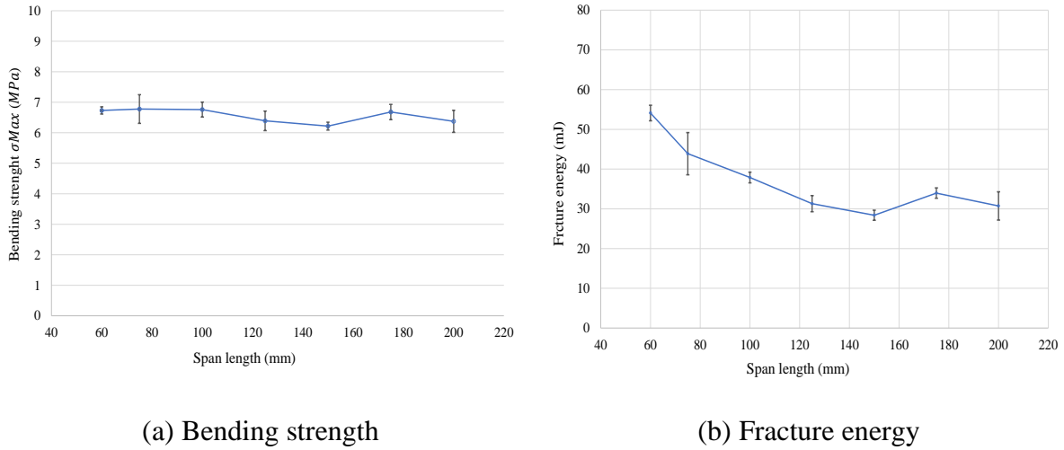
Fig. 6. Bending strength (a) and fracture energy (b) evolution as function of span length.
