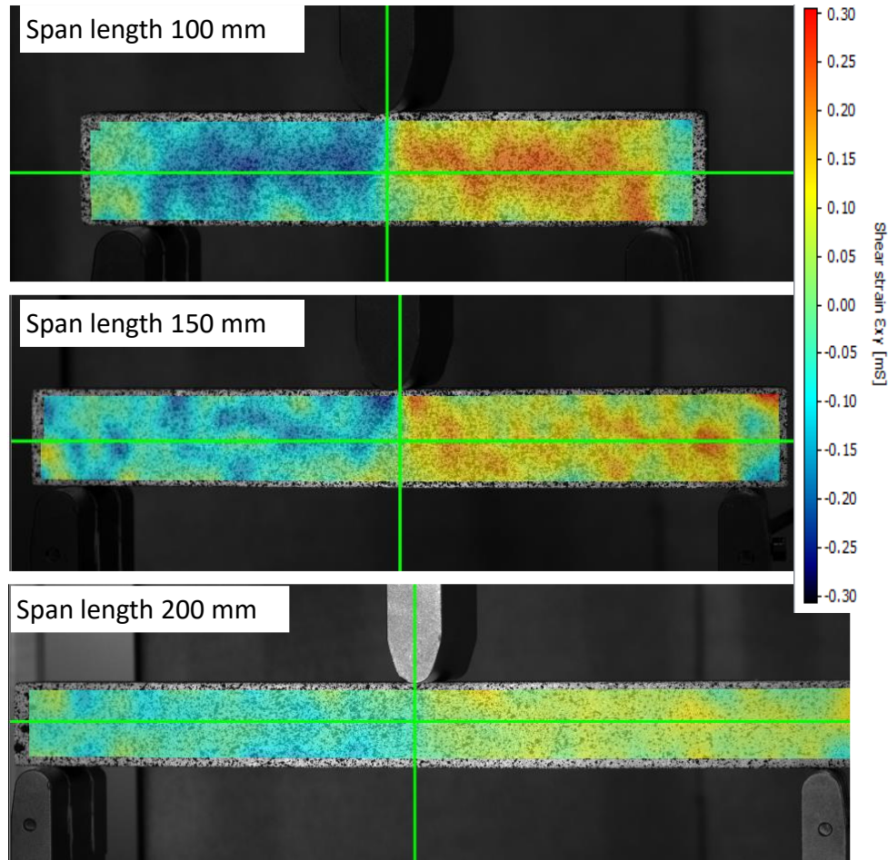
Fig. 11. Shear stain field ( \epsilon_{xy} ) measurements before fracture point at different span lengths
