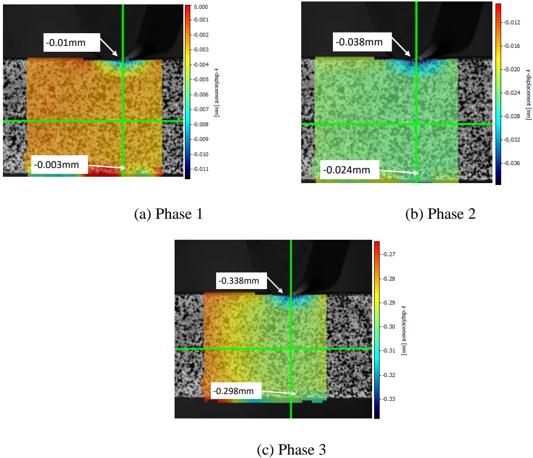
Fig. 3. Displacement fields in the loading direction of the specimen during testing.
