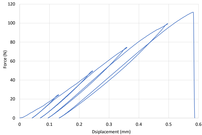
Fig. 7. Load-displacement curve of cyclic bending test performed at span length of 200 mm.
