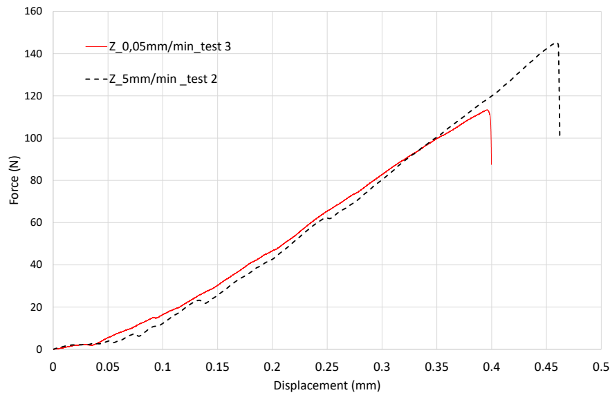
Fig. 12. Load-displacement curves as function of testing speed.
