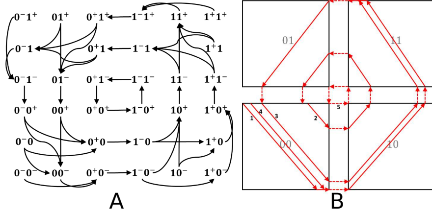
Fig 2: A: Graph of discrete domains of the HGRN of Fig 2. B: Examples of trajectories inside different discrete trajectories.
