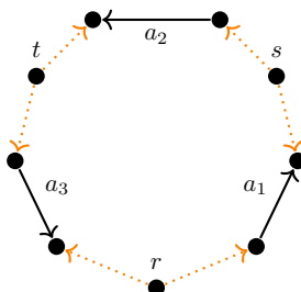
Figure 6: The clause gadget R'
