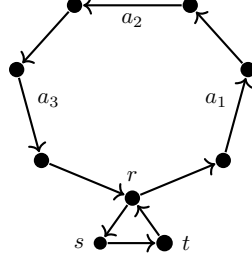
Figure 4: The clause gadget W'
