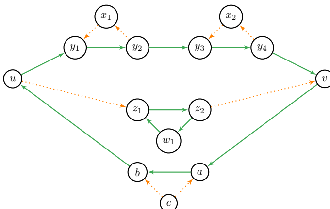
Figure 5: One of the two possible (bipartite, balanced)-arc-partitions of R[u, v, 2, 1] .
