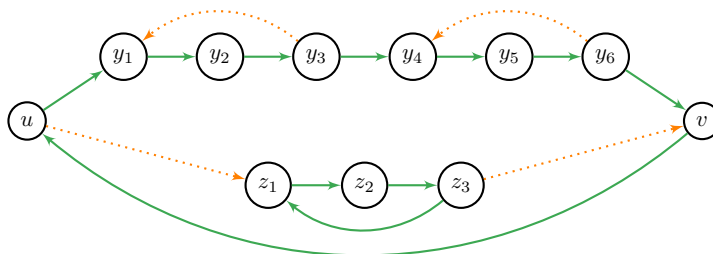
Figure 3: One of the two possible ( bipartite, cycle factor )-arc-partitions of W[u, v, 2, 1] .
