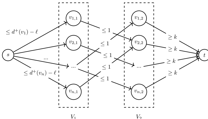
Figure 2: Construction of the network \mathcal{N}
