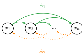
Figure 1: Construction of an ( acyclic , acyclic )-arc-partition
