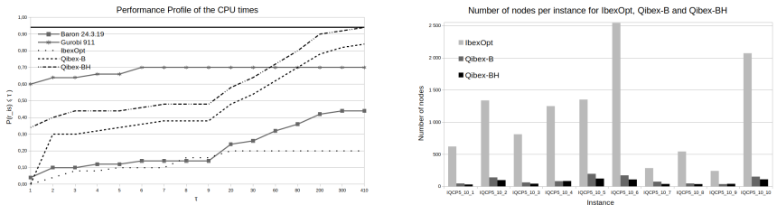
Figure 1. Performance profile of the CPU times (left) and number of nodes (right)
