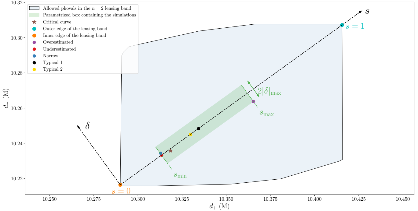
Fig. 12. Parametrization of the region in the (d_+, d_-) plane containing all the astrophysical photon ring shapes (here, for a = 0.5 and i = 45^\circ ).
