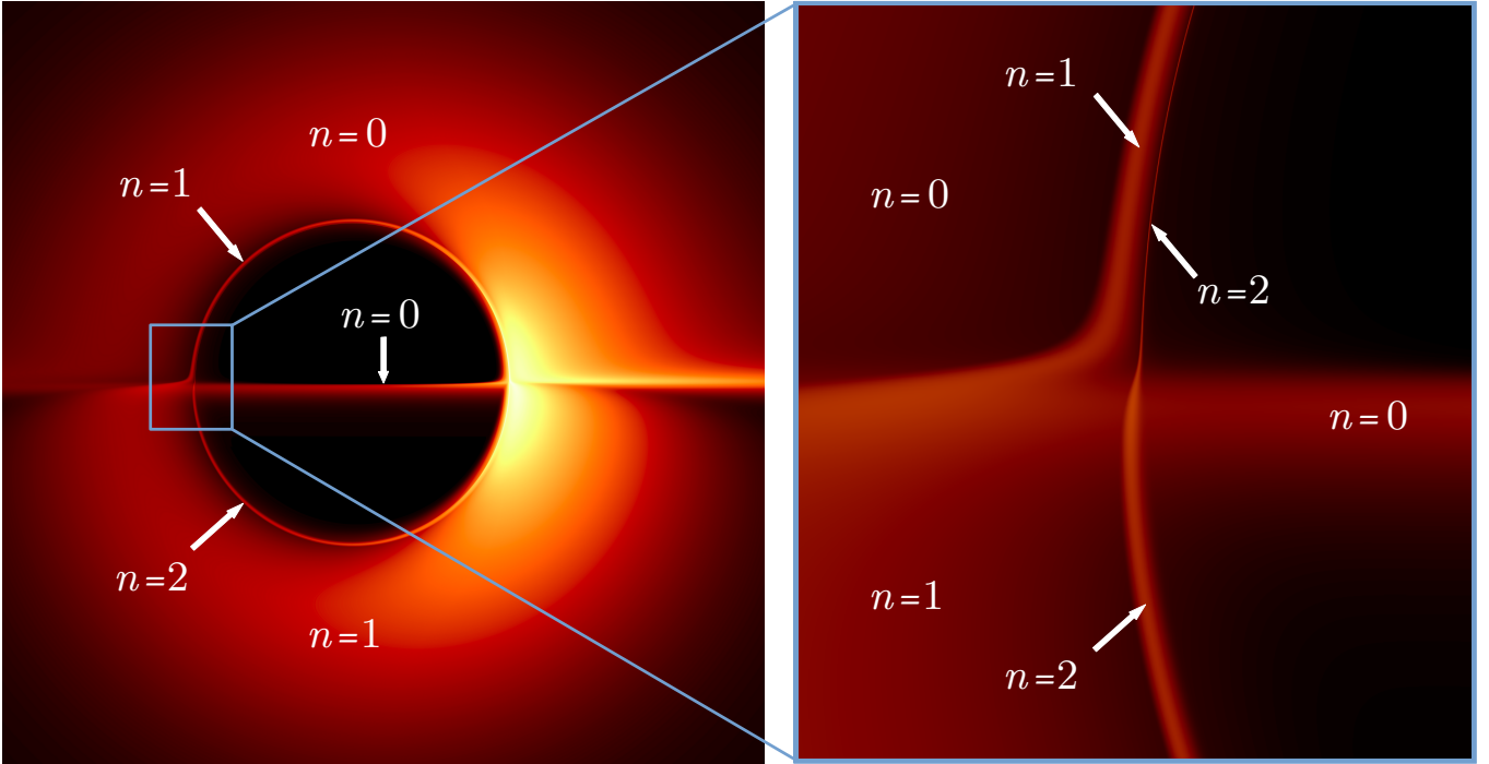
Fig. 7. Left: Gyoto log-scale image of a BH with spin a = 0.5 and inclination i = 89^\circ , surrounded by a thin disk with emission profile (Eq. (50)) with parameters \mu = r_- , \gamma = -2 , and \sigma = 1.5M . The bright horizontal line is the direct n = 0 image of the disk viewed almost edge-on. Right: zoom-in around a region with \beta \approx 0 . The width of the n = 1 subring for \beta > 0 is of the same order of magnitude as the width of the n = 2 ring for \beta < 0 .
