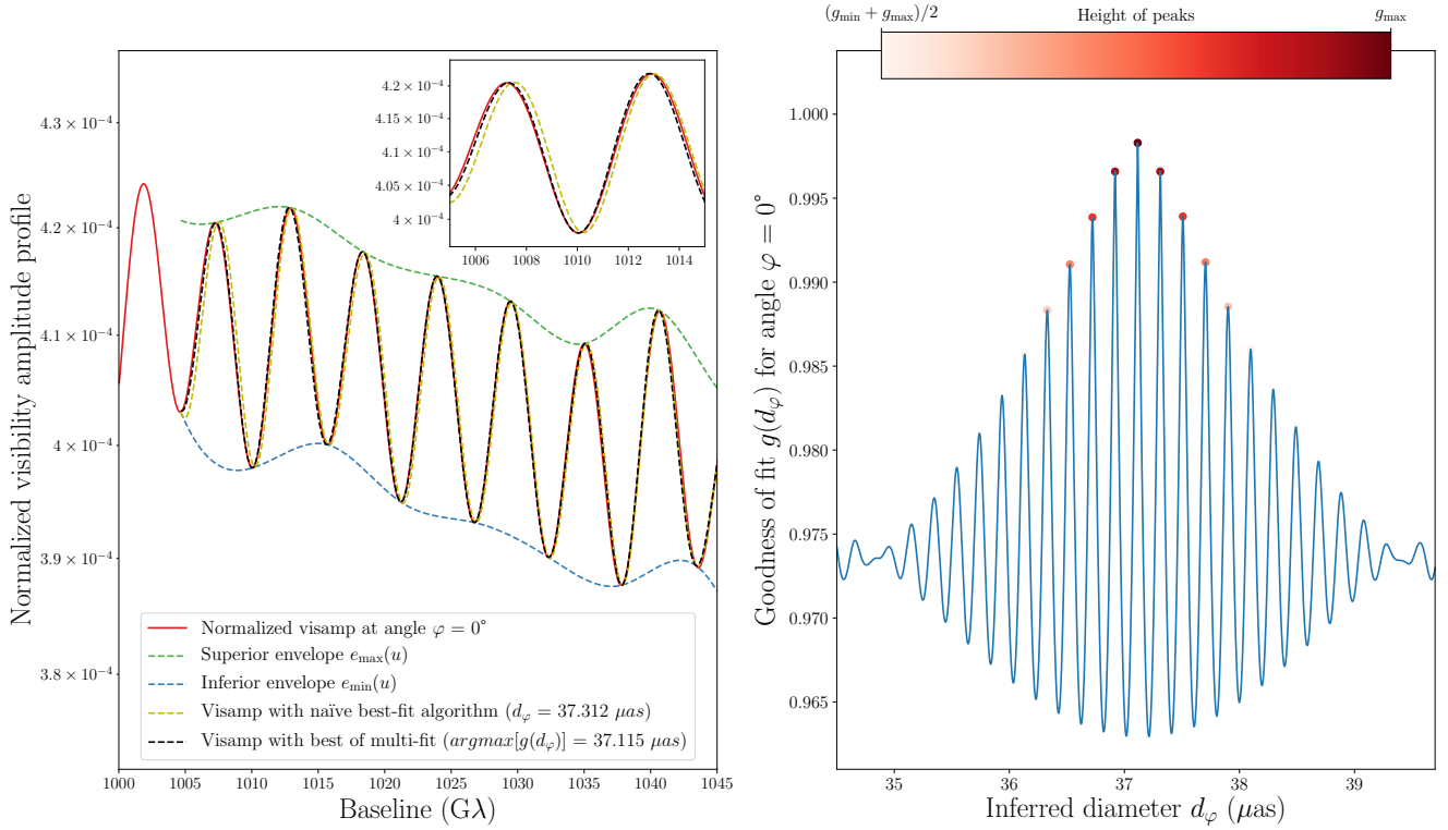
Fig. 4. Example of a model requiring a multi-peak fitting technique. Left: fit comparison: naïvely fitting the model V_{\text{fit}}(u; d) (Eq. (33)) to the visamp profile |V(u)| (solid red curve) yields an excellent but suboptimal fit (dashed yellow curve), since a better one exists (dashed black curve). Right: goodness of fit g(d_\varphi) as a function of fitting diameter (Eq. (36)). The absolute best-fit corresponds to the global maximum of g(d_\varphi) , while other local maxima correspond to good but suboptimal fits. These peaks are approximately periodic with a separation \Delta d_\varphi \approx 0.2 \mu\text{as} that exactly matches 1/u_w , since our baseline window is at u_w \sim 1000 G\lambda .
