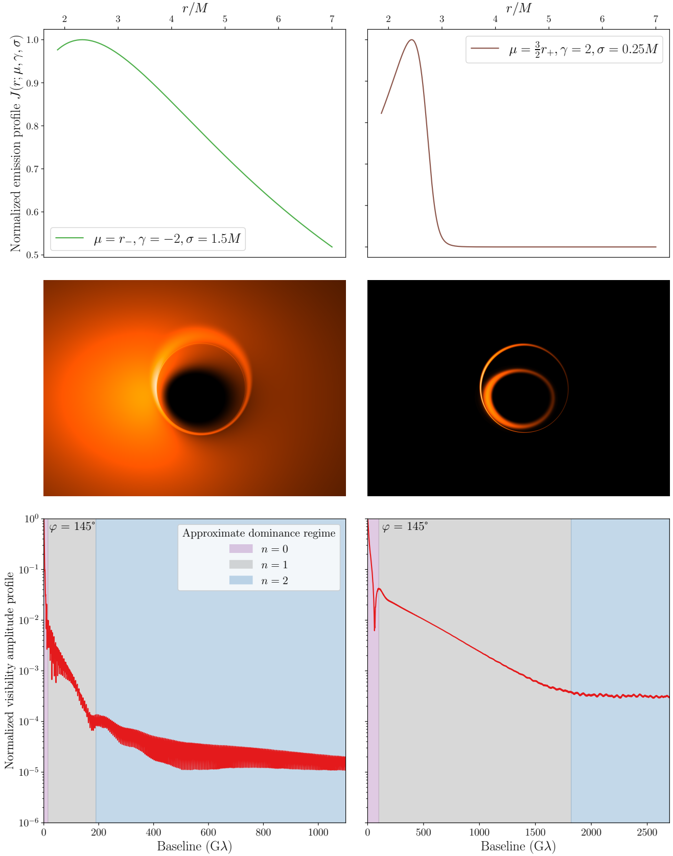
Fig. 9. Impact of the emission profile on the observed ring thickness and baseline domains. We show two extreme cases: ( Left ) A broad emission profile, leading to large rings and an early transition between n = 1 to n = 2 regimes in the visibility amplitude profile with b_2(145^\circ) \approx 200 G\lambda . ( Right ) A highly peaked emission profile, leading to thin rings (the n = 2 subring is not even visible in the image) and a late transition between the n = 1 and n = 2 regimes with b_2(145^\circ) \gtrsim 1800 G\lambda .
