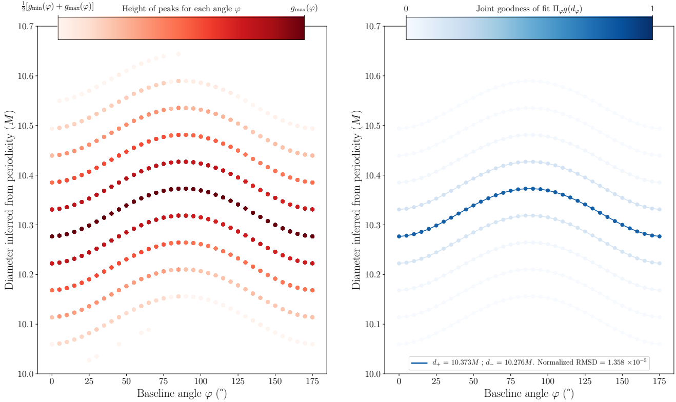
Fig. 5. Example of a successful circlipse fit and Kerr hypothesis test. Left: every 5^\circ , we determine the possible diameters d_\varphi of the n = 2 ring by maximizing the goodness-of-fit measured g(d_\varphi) (Eq. (36)). For each angle \varphi , we obtain a periodic set of diameters separated by \Delta d_\varphi \approx 1/u_w , with likelihood proportional to g(d_\varphi) and indicated by the coloring of the data point. Right: circlipse fit for each of the possible rings. The darkest circlipse is most likely to be the true shape of the image ring, since the corresponding “joint goodness of fit” far exceeds that of the other solutions.
