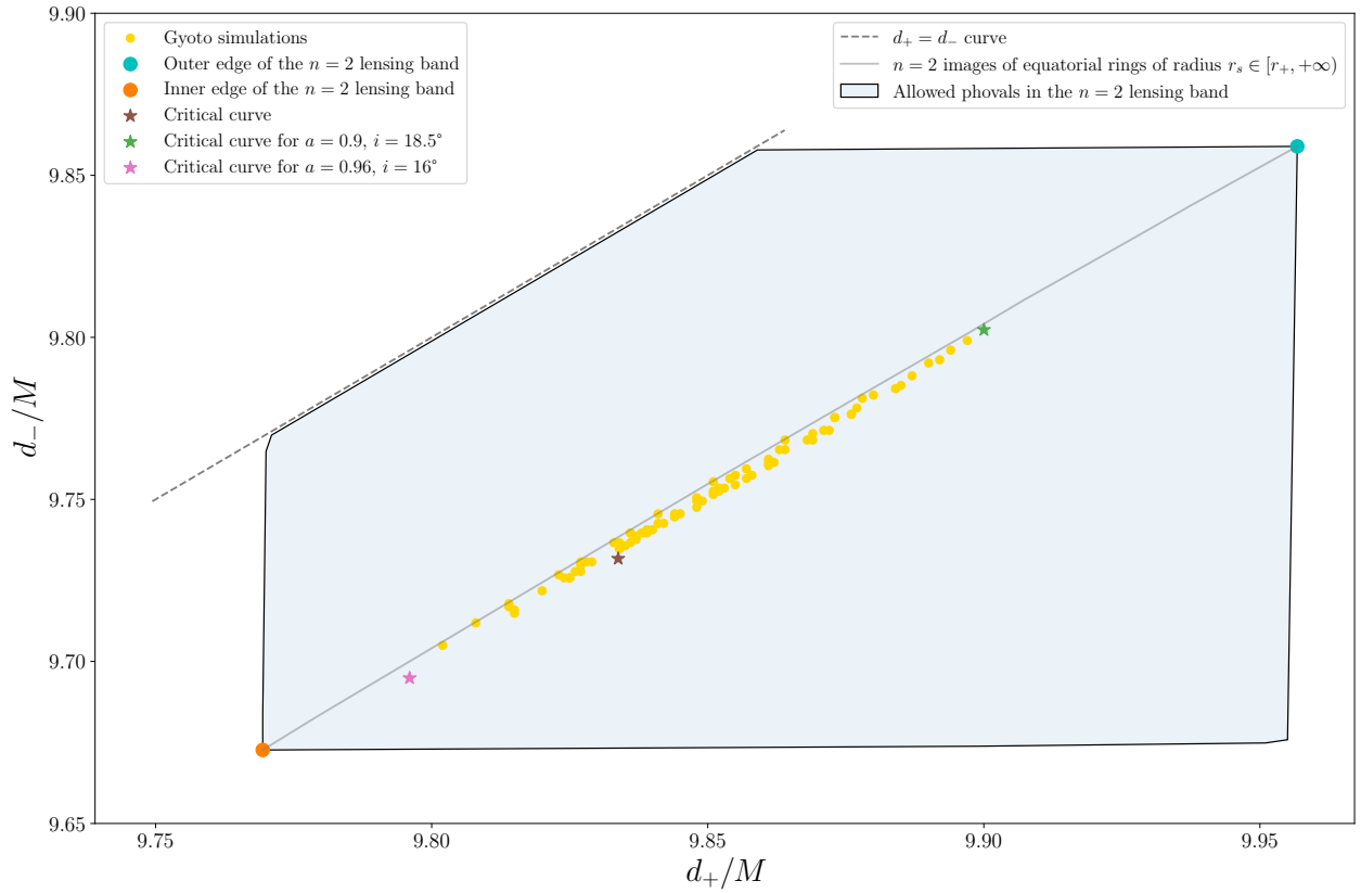
Fig. 11. Results of the survey of emission profiles in the best-guess case for M87* with spin a = 0.94 and inclination i = 17^\circ .
