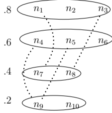
(c) The assertions of \mathcal{WA}_3
