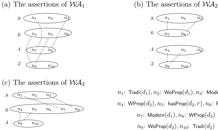
Figure 2: The compatible bases of \mathcal{A}_\triangleright : the assertions (grouped by certainty degree), and the conflicts (dotted lines).
