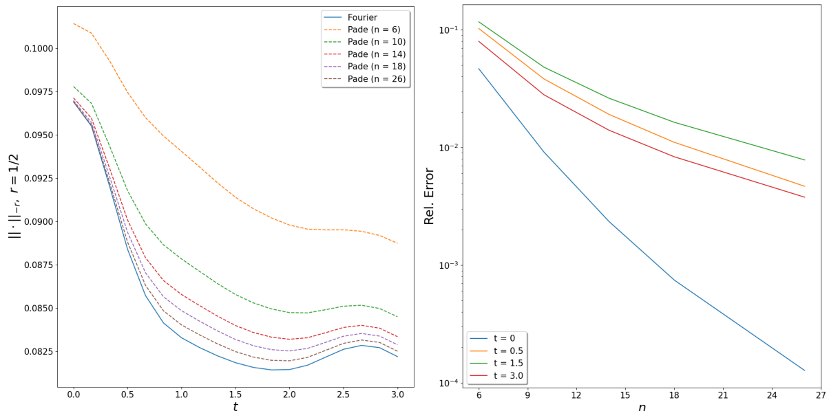
Figure 3: Convergence in Padé order for the computation of the mix-norm in a setting of fluid mixing by a time-independent slip velocity.
