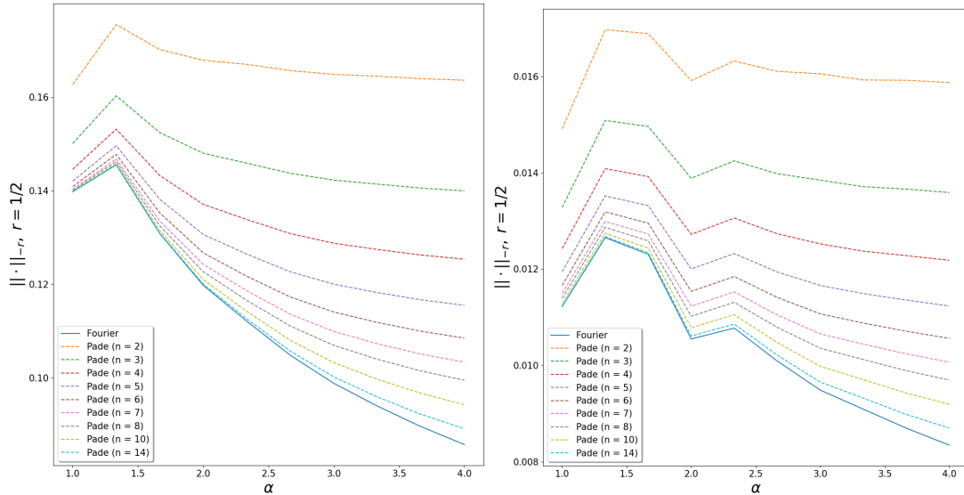
Figure 1: Mix-norm \|\cdot\|_{-r} with r = \frac{1}{2} . “Fourier” denotes the norm result when using the Hilbert basis of eigenfunctions, while the “inner product” values correspond to the inner-product of the Riesz representant u[c] in (12), and where the n value denotes the order of Padé approximation used in the computation of (17). Left: disc domain; Right: annular region
