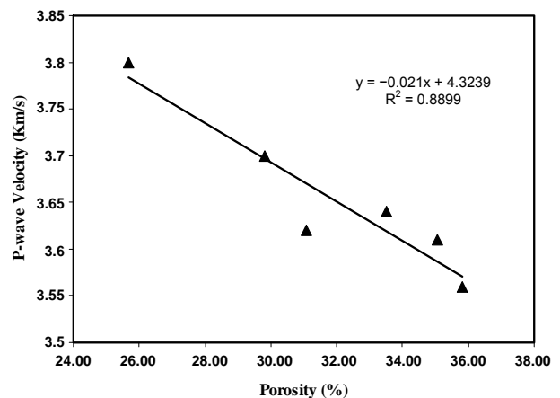
Figure 3. P-wave velocity versus porosity for dry samples.
