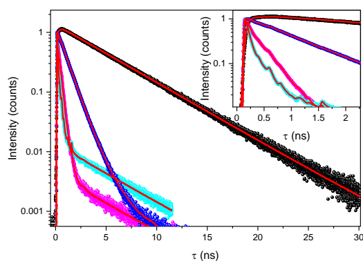
Fig. 3. Fluorescence decay of parent BDP (black, \lambda_{exc} = 495 nm, \lambda_{em} = 535 nm), BDP-C 60 dyad (pink, \lambda_{exc} = 495 nm, \lambda_{em} = 535 nm), BDP-C 60 -DSBDP triad (cyan, \lambda_{exc} = 495 nm, \lambda_{em} = 535 nm; blue, \lambda_{exc} = 495 nm, \lambda_{em} = 650 nm) in benzonitrile.
