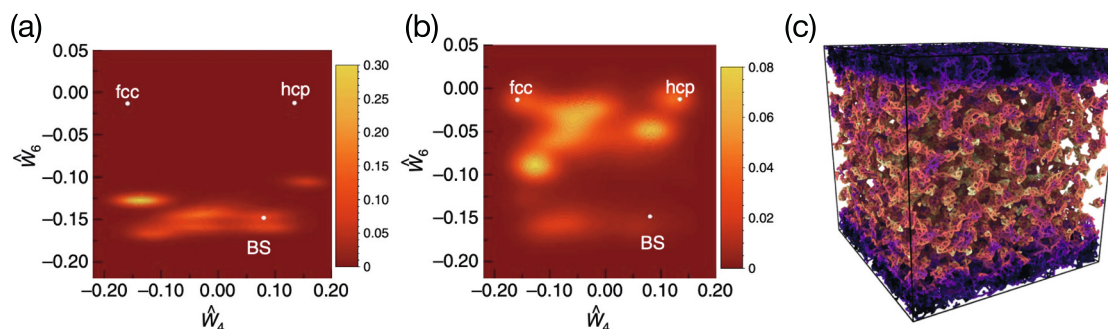
Fig. 20. Bond orientational parameters heatmaps for (a) low \text{Ca(OH)}_2 concentration potential showing high intensity at Bernal spiral (BS) packing and (b) high \text{Ca(OH)}_2 concentration potential showing high intensity in hcp or fcc crystal both at volume fraction 0.052. (c) Snapshot of the surface growth model for high \text{Ca(OH)}_2 concentration potential. The dark colour indicates higher density crust close to cement grain surfaces. Reproduced (a) and (b) from ref. [88] and (c) reprinted with permission from ref. [89]. Copyright 2020 American Chemical Society.
