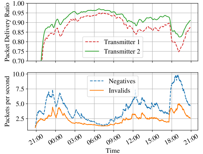
Figure 4. Packet delivery ratio and interference
