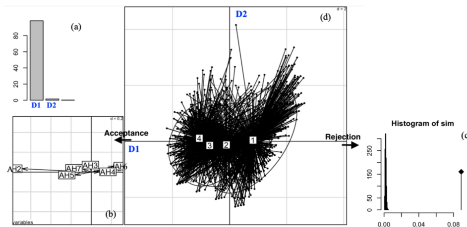
Figure 1. Between-class analyses of questions related to human evolution, depending on students declared degree of religious belief. (a) Histogram of eigenvalues of the axes D1, D2 and D3 (b) Correlation circles (c) Monte Carlo randomisation test (d) Distribution of the groups of students depending on their degree of religious belief (1 for strong belief, 4 for no or little belief declared)
