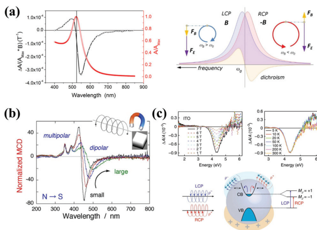
Figure 25. (a) Left, MCD/absorbance spectrum of gold nanoparticles, with MCD y-cross-over at the LSPR wavelength. Right, schematic showing the differing response for RCP and LCP light, due to different electric ( F_E ) and magnetic ( F_B ) contributions of the Lorentz force on the electrons. Adapted with permission from [234], Copyright 2013, American Chemical Society. (b) MCD spectra for silver nanocubes of varied size, exhibiting dipolar and higher-order multipolar resonances. MCD dipolar response decreases with increased size, but multipolar effects are less size-dependent. Adapted with permission from [236], Copyright 2018, Elsevier. (c) Electron polarisation scheme for Doped-ITO nanoparticles. Top left, MCD spectrum at different field strengths is given in dashed coloured lines. Right, the temperature dependency of the MCD signal. Lastly the schematic of the conduction band splitting due to the angular momentum of the magnetoplasmonic modes due to RCP and LCP excitation. Adapted with permission from [237], Copyright 2018, Springer Nature.
