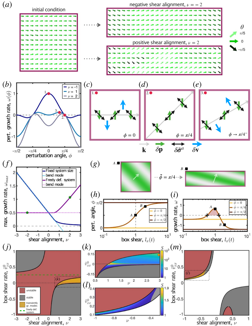
Figure 3. Linear stability of the polar-only system, \beta = 0 . (a) Simulations of a freely deforming system with fixed-magnitude polarity and extensile active stresses, for two different values of the shear alignment parameter \nu . (b) Growth rate \omega of a perturbation with angle \phi in a system with a fixed polarity magnitude (i.e. \text{sgn}(A) = -1 and \tau \rightarrow 0 ) for three different \nu values. (c)–(e) Schematics illustrating the perturbation dynamics for three different \phi (section 4.1). (f) Perturbation growth rate maximized across all wave vectors, \omega_{\max} , for fixed system (blue) and freely deforming system (purple). The dashed lines represent the growth rates of the respective bend modes ( \phi = 0 ). Green stars correspond to the \nu values used for the simulations in panel a. (g) Illustration of the change of the wave vector \mathbf{k} measured in the lab frame (arrow) for a given co-deforming mode \bar{\mathbf{k}} as the system is sheared from l_x(t) = 1 (A) to l_x(t) = 2 (B; compare equations (25) and (26)). (h) Perturbation angle \phi measured in the lab frame versus the box shear l_x , for three different co-deforming angles \bar{\phi} . (i) Change of the growth rates \omega of three co-deforming perturbation modes (same as in panel (h) as the box width l_x changes during the box deformation. The co-deforming \bar{\phi} = \pi/4 mode transiently experiences a positive growth rate (positive \omega values between ‘+’ signs). Fixed polarity magnitude, \bar{v}_{xx}^0 = 1/8 , \nu = 3 . (j)–(m) Stability phase diagrams for (j), (k) fixed polarity magnitude and (l), (m) zero preferred polarity magnitude with \tau = 10 , where red, gray, and yellow respectively indicate unstable regions, stable regions, and stable regions with transiently growing modes. The green dashed line in (j) represents the deformation rate of the freely deforming system. Black lines marking phase boundaries are analytical curves derived in appendix B.3. (k)–(l) Maximal perturbation amplification factor S in the stable regions with transiently growing modes. Orange star in (k) corresponds to the parameters used for panel i.
