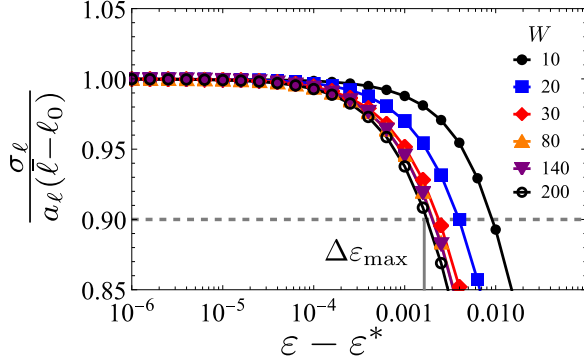
FIG. 9. \Delta\varepsilon_{\max} in Fig 6 is defined as the strain range where the ratio \sigma_\ell/(\bar{\ell} - \ell_0) shows a deviation of less than 10% from its value a_\ell defined very close to the transition point (appendix C).
