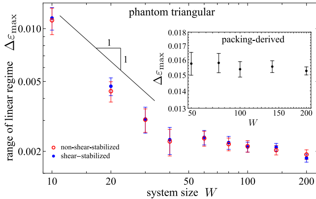
FIG. 6. Plot of the isotropic strain range \Delta\varepsilon_{\max} = \varepsilon_{\max} - \varepsilon^* within which the \bar{\ell}_{\min} function scales linearly with \sigma_\ell , shown here for increasing system size W for phantom triangular networks, and for shear-stabilized packing-derived networks (inset). In both cases, we use z = 3.2 and rope-like potentials. The range \Delta\varepsilon_{\max} is quantified as explained in appendix G and Figure 9. While for W \gtrsim 60 , the linear range of the phantom triangular networks appear to show a weak power-law dependence on W , there is no significant dependence on system size for packing-derived networks. Error bars indicate the standard error of the mean.
