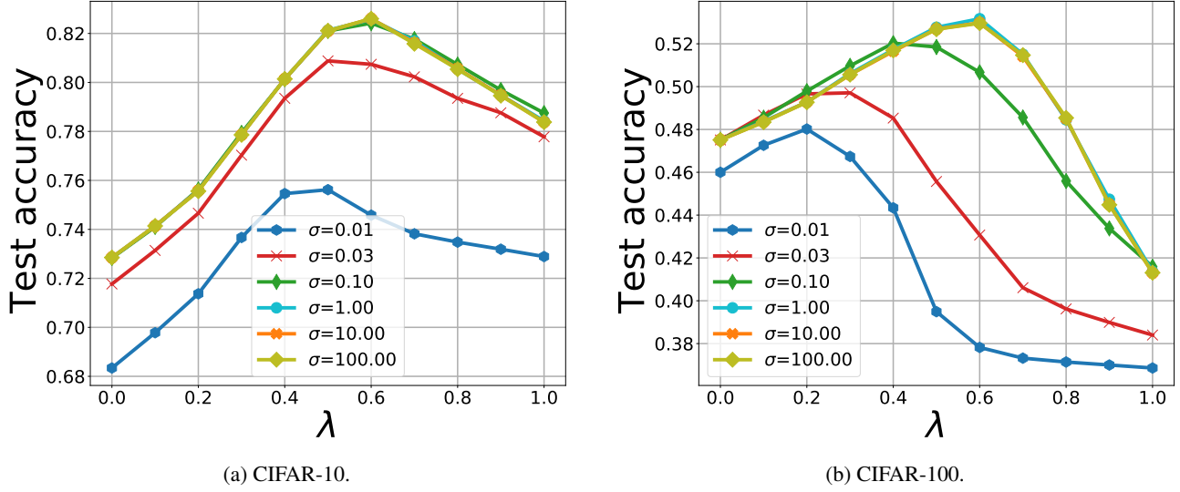
Figure 7. Test accuracy vs the interpolation parameter \lambda for different values of the kernel scale parameter \sigma .
