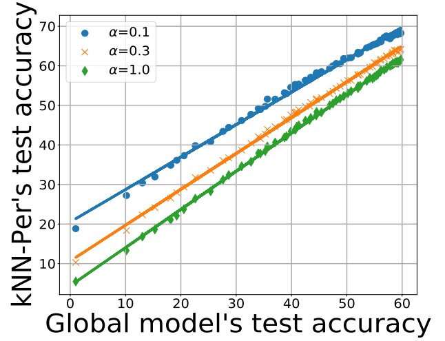
(b) CIFAR-100.
