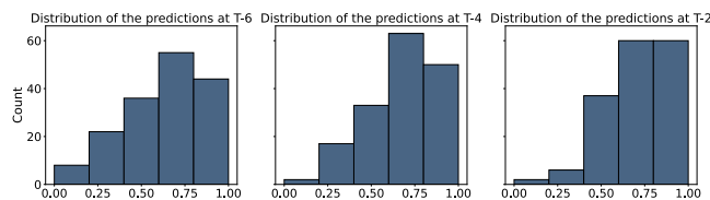
Fig. 5: Performance of the model at T-6, at T-4, and T-6
