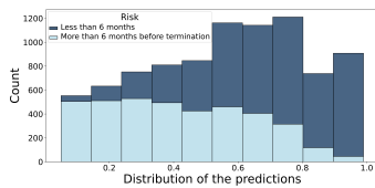
Fig. 3: Distribution of the predictions by class
