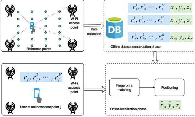
Figure 1. RSS Fingerprinting
