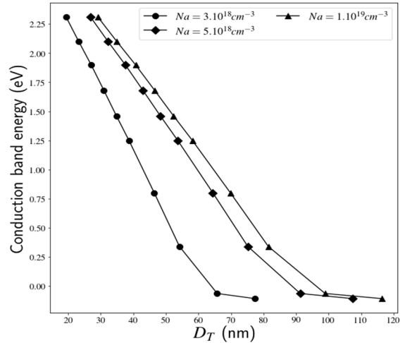
Fig. 7. Simulated variations of the conduction band energy level versus the well spacing D_T for different P-GaN doping concentrations
