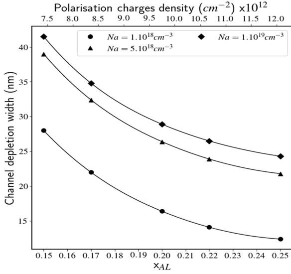
Fig. 5. Simulated variations of the channel depletion width as a function of the aluminum content x_{\text{Al}} and the polarisation charges density for different P-doping concentrations
