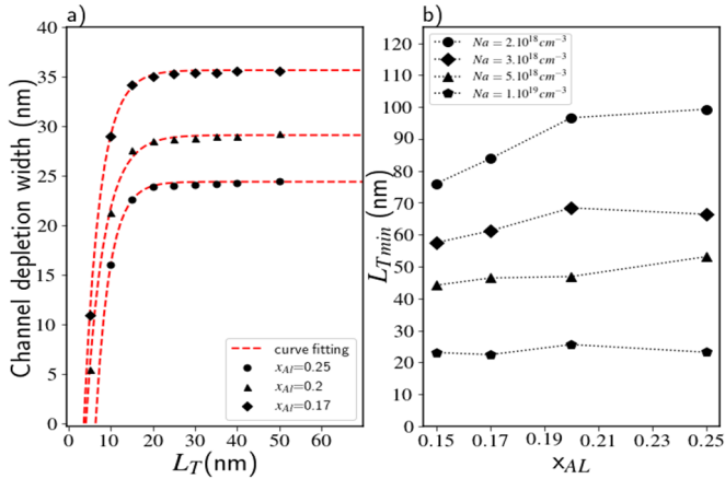
Fig. 6. a) Simulated variations of SCR width as a function of L_T for a 1 \times 10^{19} \text{ cm}^{-3} P-GaN doping concentration and different aluminum contents x_{\text{Al}} ; b) L_{T\text{min}} variations as a function of x_{\text{Al}} for different P-doping concentrations ( \epsilon_T = 100 \text{ nm} )
