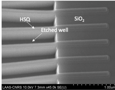
Fig. 11. MEB view of the multiwells along the gate after HSQ e-beam lithography and AlGaIn/GaN BCl 3 etching.
