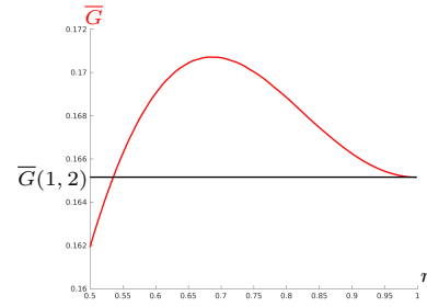
Fig. 5. The map r \mapsto \bar{G}(r, S^{in}) with \bar{G} defined by (14), f(S) = 4S/(5 + S) , a = 0.6 and S^{in} = 2 .
