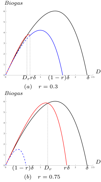
Fig. 3. The curves of the functions D \mapsto G_1(S^{in}, D, r) (in blue), D \mapsto G_2(S^{in}, D, r) (in red) and D \mapsto G_{chem}(S^{in}, D) (in black), with D_r = D_r(S^{in}) , S^{in} = 7 , f(S) = 4S/(5 + S) and a = 0 .
