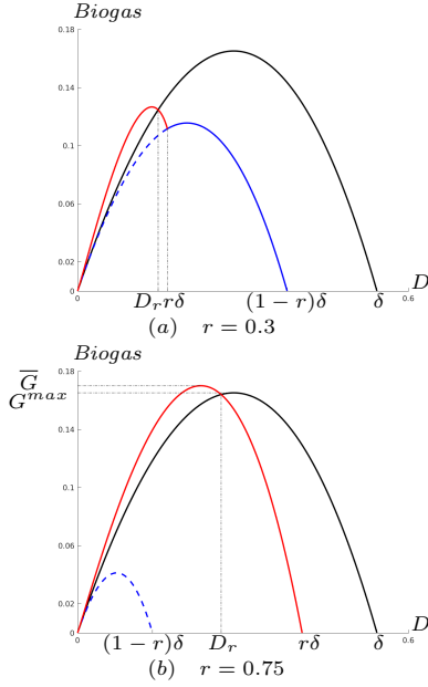
Fig. 4. The curves of the functions D \mapsto G_1(S^{in}, D, r) (in blue), D \mapsto G_2(S^{in}, D, r) (in red), and D \mapsto G_{chem}(S^{in}, D) (in black), with G^{max} = G^{max}(S^{in}) defined by (13), \bar{G} = \bar{G}(r, S^{in}) defined by (14), S^{in} = 2 , f(S) = 4S/(5 + S) and a = 0.6 .
