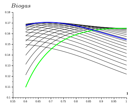
Fig. 6. Curves r \mapsto G_2(S^{in}, D, r) for different values of D , with f(S) = 4S/(5 + S) , a = 0.6 and S^{in} = 2 . In blue, the one for D \simeq 0.213 such that \max_r \bar{G}(r, S^{in}) = \max_r G_2(S^{in}, D, r) . In green, the one for D \simeq 0.283 such that G^{max}(S^{in}) = G_{chem}(S^{in}, D) .
