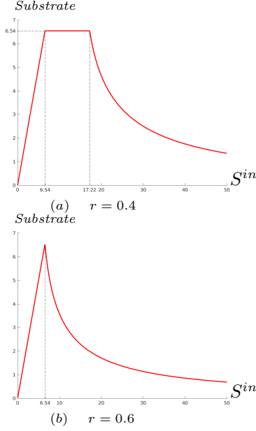
Fig. 1. The curve of the output substrate concentration with respect to S^{in} , with f(S) = 4S/(5 + S) , D = 1 and a = 0.6 . In (a): \lambda(D/(1-r) + a) \approx 6.54 and \lambda(D/r + a) \approx 17.22 . In (b): \lambda(D/r + a) \approx 6.54 .
