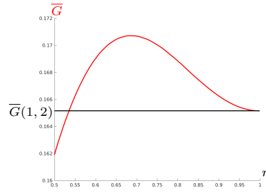
Fig. 5. The map r \mapsto \bar{G}(r, S^{in}) with \bar{G} defined by (14), f(S) = 4S/(5 + S) , a = 0.6 and S^{in} = 2 .
