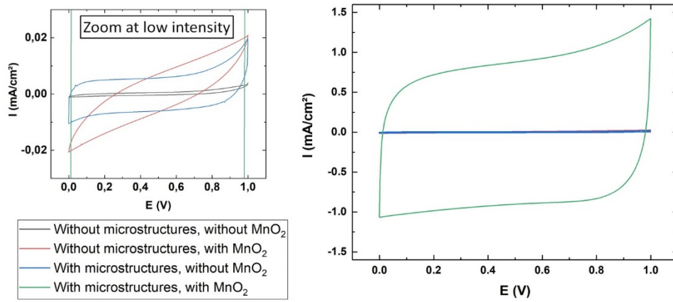
Fig. 8 | CVs at 20\text{mV}\cdot\text{s}^{-1} of face-to-face \mu SCs, with [PVDF]/EMI/TFSI 17/83 wt % ionogel as electrolyte, with 3D microstructured electrodes or not and covered with MnO 2 or not.
