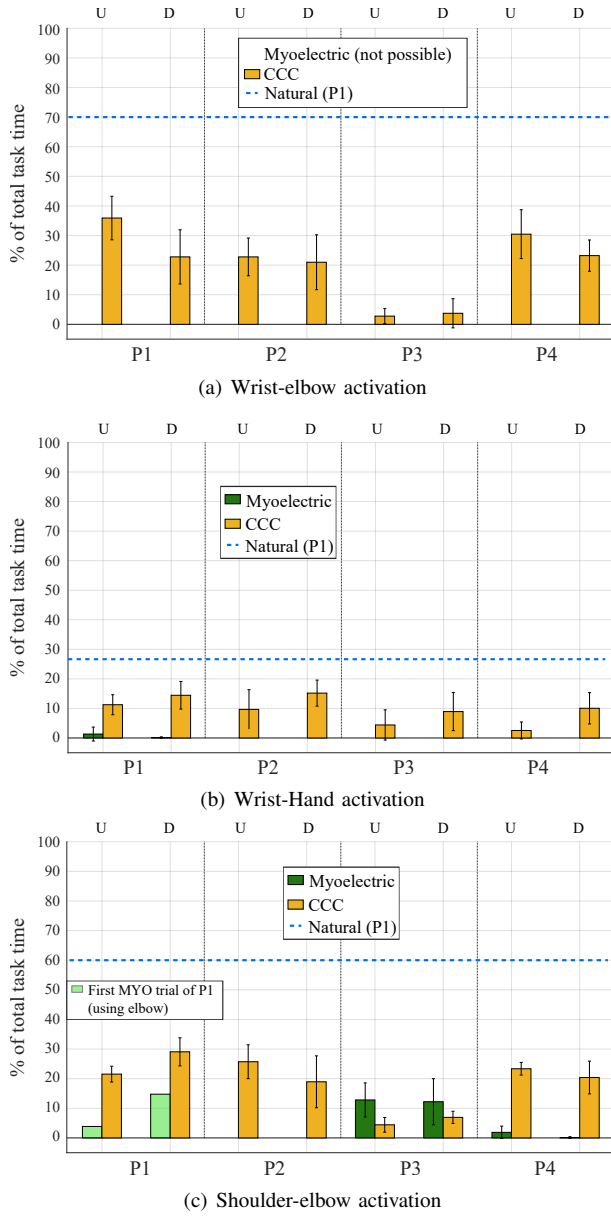
Fig. 7: Simultaneous activation of prosthetic and prosthetic-human joints: (a) wrist and elbow, (b) wrist and hand, (c) shoulder and elbow. For P1, the first trial is set apart (light green), since it was the only one for which the elbow was activated. U: upwards; D: downwards motions.
