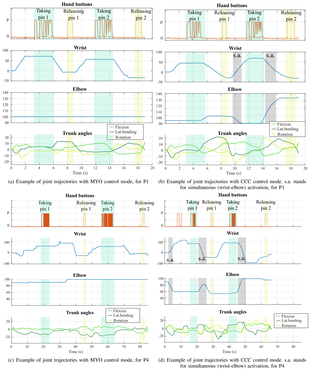
Fig. 4: Example of joint trajectories and hand activation from one upwards motion of P1 (a and b) and one upwards motion of P4 (c and d).
