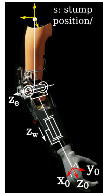
Fig. 2: Prosthesis model used to obtain the prosthesis position error from the stump orientation.
