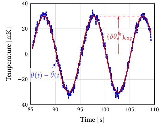
Figure 7 Efficiency of the synchronous demodulation to reach (\delta\theta_e^{f_0})_{\text{exp}} (PA6.6, T_0 = 313 K, f_0 = 0.1 Hz, Figure 5(a).
