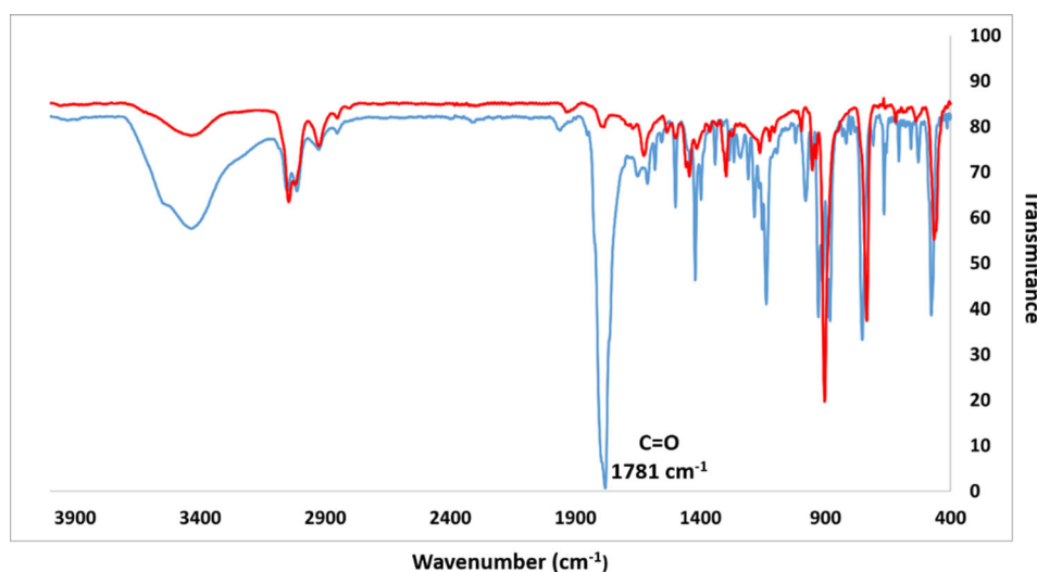
Fig. 6 FTIR spectra (KBr pellets) of a carbonylated precursor and of nonacene 1 . The spectrum of the precursor 7b is in blue, with a strong CO peak at 1781 cm -1 and that one of the resulting nonacene 1 is in red, after 1 min. heating at 350 °C in glovebox.
