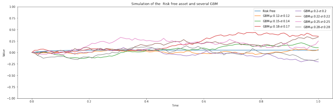
Figure 1: Time evolution of the return of the discretized trajectories associated to the assets of the synthetic portfolio (CIR + GBM).
