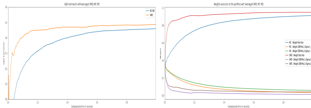
Figure 4: Evolution of the V@R estimation (left) of the portfolio with the computational time of the SMD and of the MC-MD p_\lambda with \lambda = 0.95 and \alpha = 0.05 . The composition of optimal portfolio (right) converges to similar values as represented on the right with SMD and MC-MD but with a different cost in computational time.
