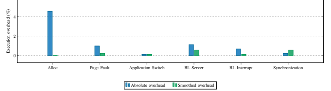
Fig. 8. Absolute overhead of the safety net compared to the smoothed overhead introduced at run-time.
