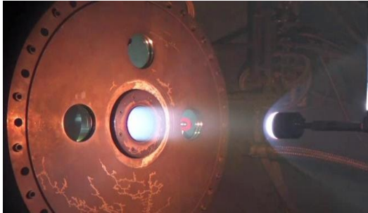
Fig. 14. Test environment for stagnation flow test.
