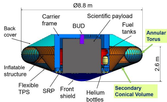
Fig. 9. Mars scenario HIAD entry vehicle.
