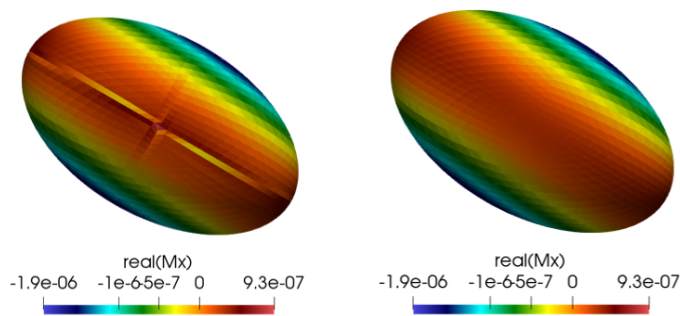
Figure 7. Single-body example, HC object: \text{Re}(\mathbf{M} \cdot \mathbf{e}_x) in the Oxz plane for \eta = 10^{-6} , computed without (left) or with (right) suppression of the vanishing static double-layer operator \mathbf{D}_\ell^{ab} in the loop-loop interactions of the PMCHWT problem.
