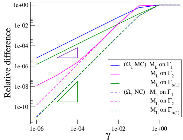
Figure 11. Multi-body example: convergence of the relative differences of M_L (in L^2(\Gamma_a) norms) on \Gamma_1 , \Gamma_2 and \Gamma_{\alpha(1)} , where \Omega_1 is either NC or MC.
