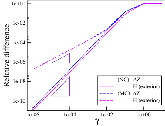
Figure 6. Single-body example, NC or MC body: convergence plots for the relative differences in the impedance variation and external magnetic field. The triangles show O(\eta) and O(\eta^2) rates for visual comparison with theoretical orders of convergence.
