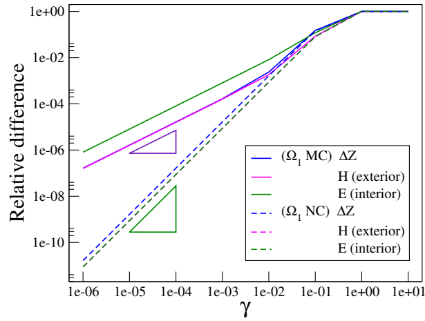
Figure 10. Multi-body example: convergence of the relative differences of \Delta Z and the relative differences of \mathbf{H} in L^2(S_0) norm and \mathbf{E} in L^2(S_1) norm, where \Omega_1 is either NC or MC.
