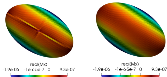
Figure 7. Single-body example, HC object: \text{Re}(\mathbf{M} \cdot \mathbf{e}_x) in the Oxz plane for \eta = 10^{-6} , computed without (left) or with (right) suppression of the vanishing static double-layer operator \mathbf{D}_\ell^{ab} in the loop-loop interactions of the PMCHWT problem.
