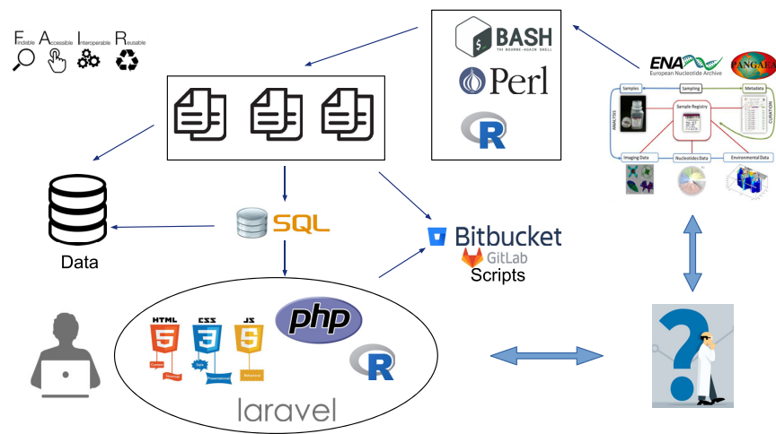
Figure 6. OGA2 processing. To answer to the FAIR principles (Findability, Accessibility, Interoperability, and Reusability), the processing of OGA2 server is the following: the metadata (sample gene abundance tables, environmental context and gene catalogues) are collected from a data warehouse such as ENA, PANGAEA or companion websites. All data objects are preprocessed using bash, perl or R scripts to generate the files for database integration and BLAST databases are generated from sequence files. Laravel requests allow to query the different datasets and the application server communicates with the user through an Apache 2 HTTP server to display results. Every week an OGA2 database dump is done to save the data to a remote backup server. In order to facilitate updates and collaborative work, the scripts are hosted under bitbucket and gitlab.
