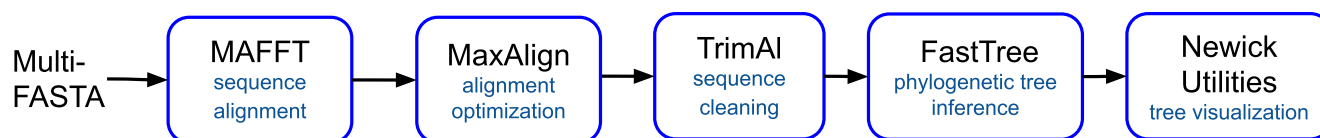
Figure 2. Phylogenetic pipeline. All sequences identified as homologous to the user query sequence are first aligned with MAFFT (23), the sequence alignment is treated with MaxAlign (24) to maximize the number of amino acid symbols in the alignment area and cleaned with an automated alignment trimming tool named trimAl (25). FastTree (26), with the default settings, allows to infer approximately-maximum-likelihood phylogenetic tree from the resulting alignment with the JTT (Jones-Taylor-Thornton 1992) model of amino acid evolution, and computes local support values with the Shimodaira-Hasegawa test. The tree visualization is done with Newick Utilities tools suite (27).
