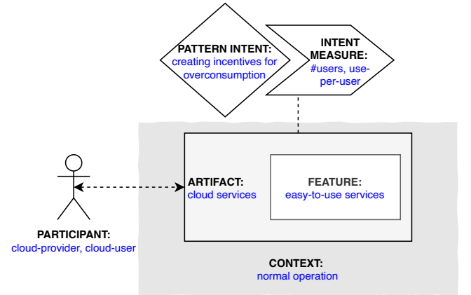
Figure 2: The Pattern Model (with a pattern example in blue text)
