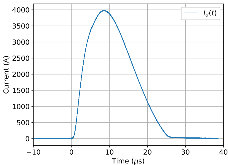
Fig. 3 Typical PJP discharge current waveform during one pulse
