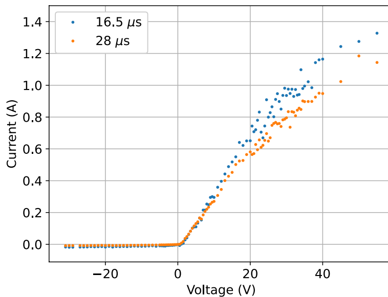
Fig. 6 Reconstructed I-V curves at 16.5 μs and 28 μs
