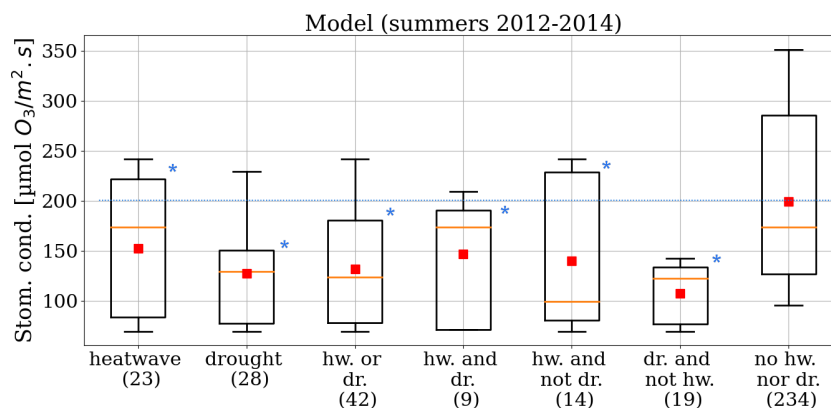
Figure 11. Same as Fig. 10 with the simulated O 3 stomatal conductance ( \mu\text{mol O}_3 \text{ m}^{-2} \text{ s}^{-1} ) by the CHIMERE model (LAIdetr/ f_{\text{SWS-dep}} experiment).
