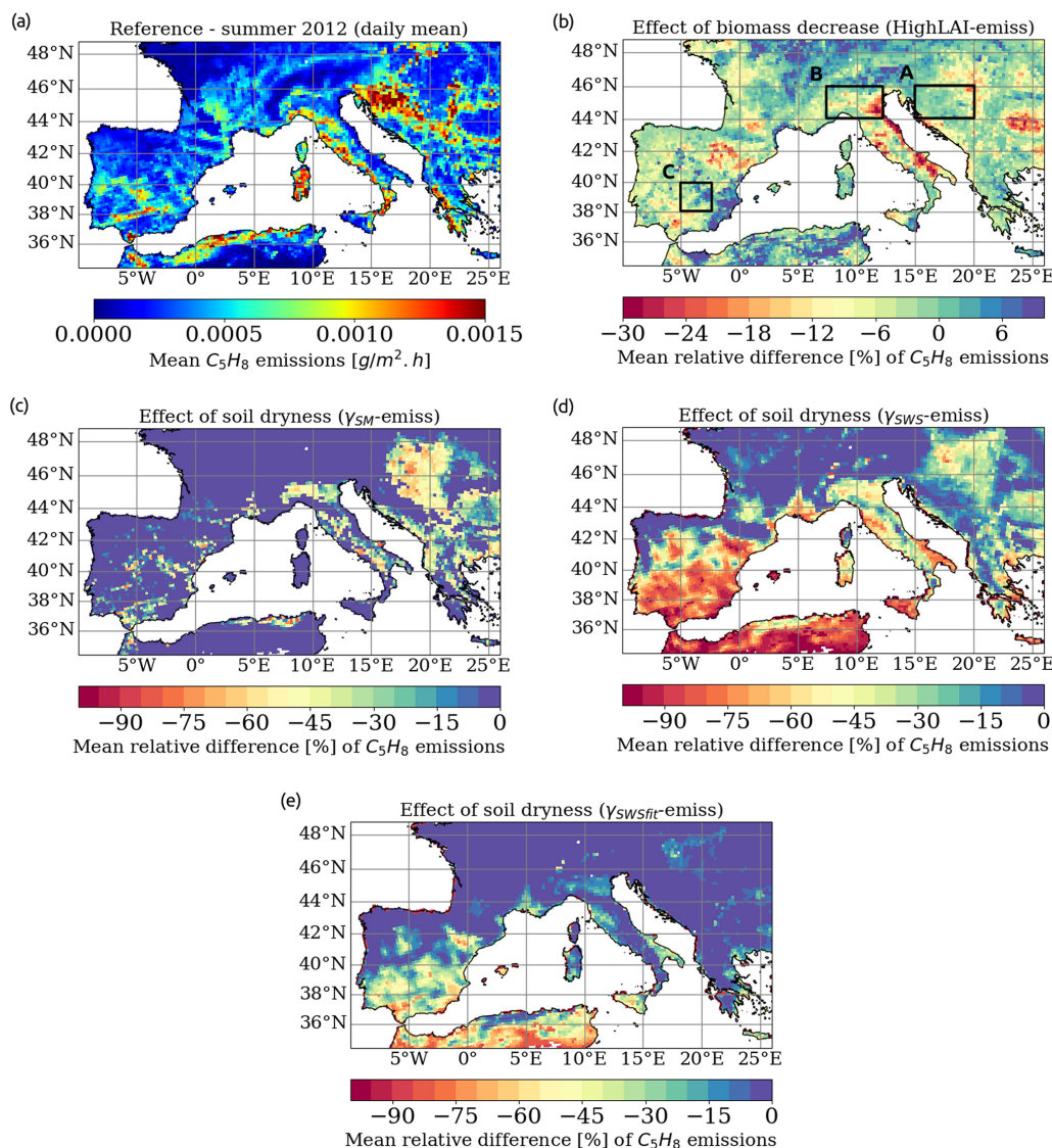
Figure 2. Summer mean (June–August, JJA) of the daily mean C 5 H 8 emissions (g m -2 h -1 ) for 2012 from the reference simulation (a). Mean relative difference (%) in C 5 H 8 emissions due to the biomass decrease and soil dryness. The relative difference is computed between the reference and HighLAI-emiss simulation to quantify the biomass decrease effect (b) and the γ SM -emiss (c), γ SWS -emiss (d), and γ SWSfit -emiss (e) simulation to quantify the soil dryness effect (for each configuration). For diagnostic purposes, areas of interest are designated within the dashed rectangles in panel (b), which are the Balkans (A), Po Valley (B), and central Spain (C).
