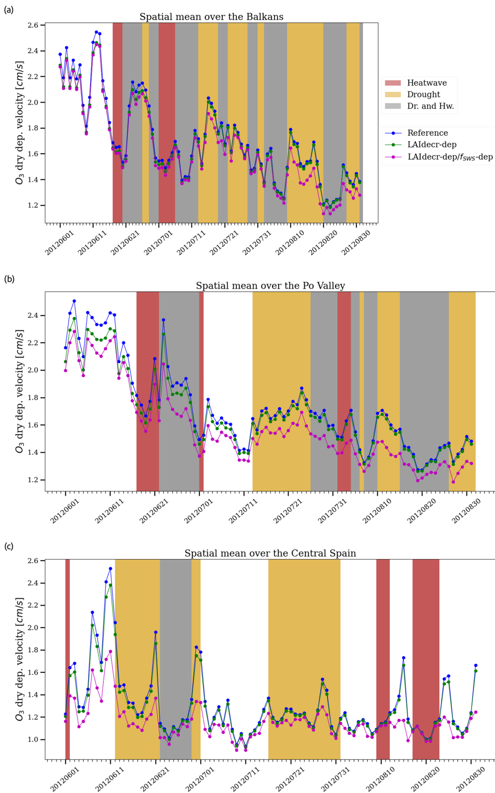
Figure 6. Daily mean O 3 dry deposition velocity ( \text{cm s}^{-1} ) during summer 2012, spatially averaged over the Balkans (a), Po Valley (b), and central Spain (c) for the different CHIMERE experiments.
