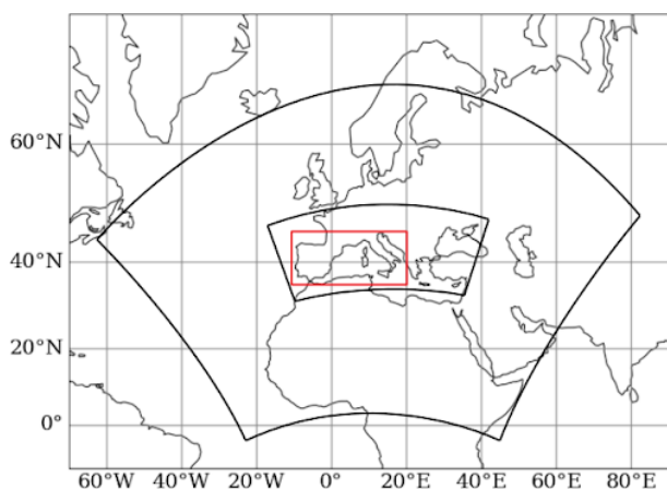
Figure 1. Domains used for the CHIMERE simulations. EUMED60 at 60 km resolution is the large domain, and the smaller nested domain is Med-CORDEX at 20 km resolution. The south-western Europe region studied here is shown in red.
