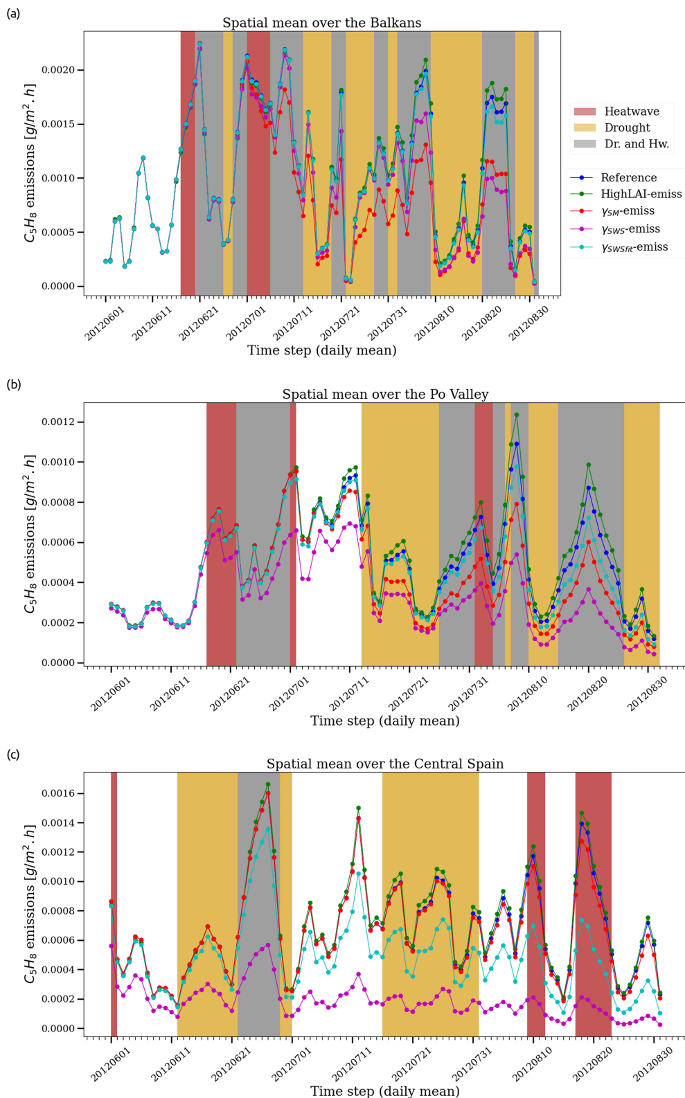
Figure 3. Daily mean C_5H_8 emissions ( g\ m^{-2}\ h^{-1} ) during summer 2012, spatially averaged over the Balkans (a), Po Valley (b), and central Spain (c), for the different MEGAN experiments. The coloured bands highlight periods of droughts and heatwaves.
