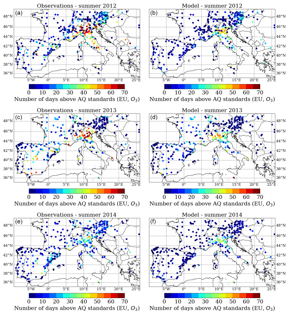
Figure 13. Number of days above the air quality threshold value from the European Union for surface O 3 (maximum daily 8 h mean of 120 µg m -3 ) over the summers of 2012, 2013, and 2014 (JJA; 92 d in total). EEA observations (left column) are compared to CHIMERE (all-emiss-dep) simulations (right column).
