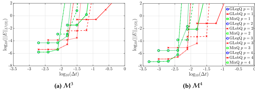
Figure 4: Influence, in the case of constant velocity and constant jacobian, of time step on the \mathcal{L}^2(\Omega) -error at T = 1 for different polynomial orders, meshes and method.
