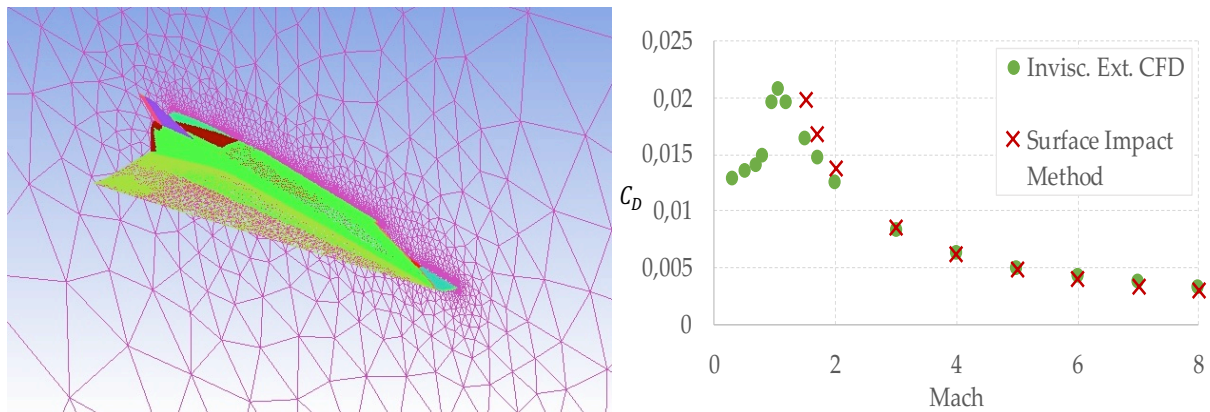
Fig. 9. Inviscid Grid (1M cells) and Drag coefficient vs Mach number
