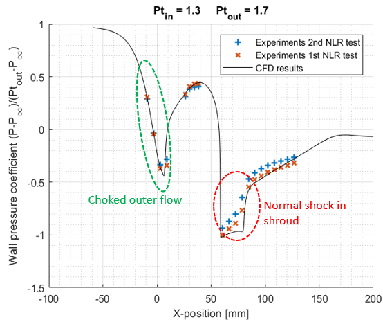
Fig. 18. Comparison between the experimental wall pressures and the wall pressure computed with CFD
