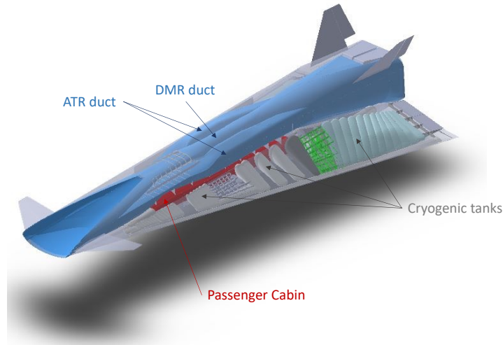
Fig. 1. STRATOFLY MR3 vehicle layout and subsystems integration
