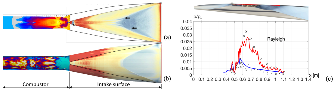
Fig. 15. Measured (a) and computed (b) wall heat flux on the lower combustor wall and on the intake. The same colormaps are used for the measured and computed images on each part but different colormaps are used for the lower combustor wall and intake. The experimental wall heat flux image for the intake is obtained from [x8] whereas those of the lower combustor wall are provided by DLR. In figure 15 experimental (symbols) and computed wall pressures, p , normalized by the free stream total pressure, p_t , are presented for a non-reacting case (blue) and a reacting case (red) along the highlighted line
