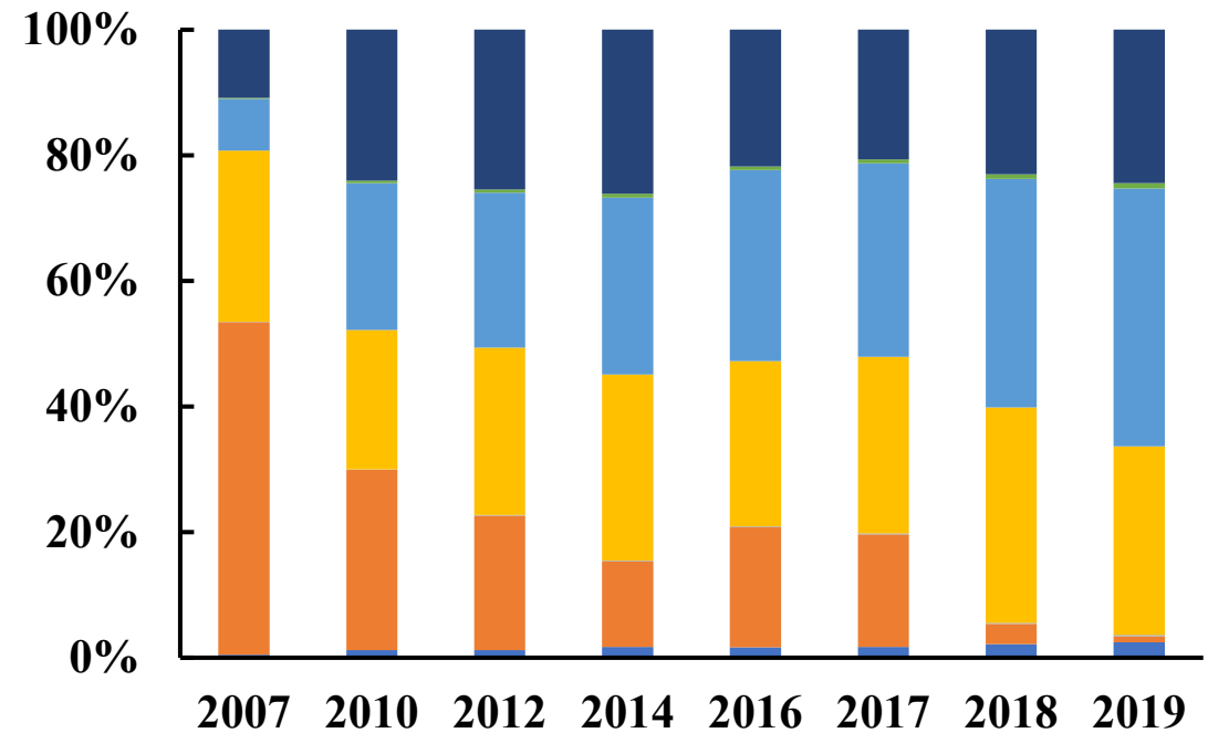
PM2.5
