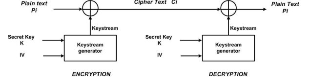
Fig. 1. General structure of a stream cipher.
