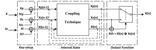
Fig. 2. Structure of CM-PCNG.
