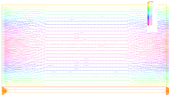
Figure 3: Velocities, f_1 = (1, -1) = f_2 , n = 9 , \alpha = 10^9
