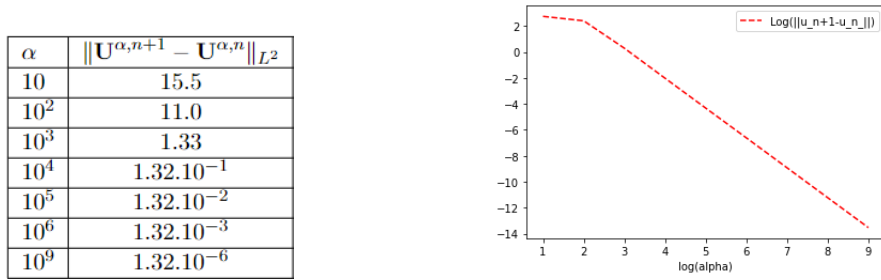
Figure 2: L2 norm of the errors and rate of convergence for n=100
