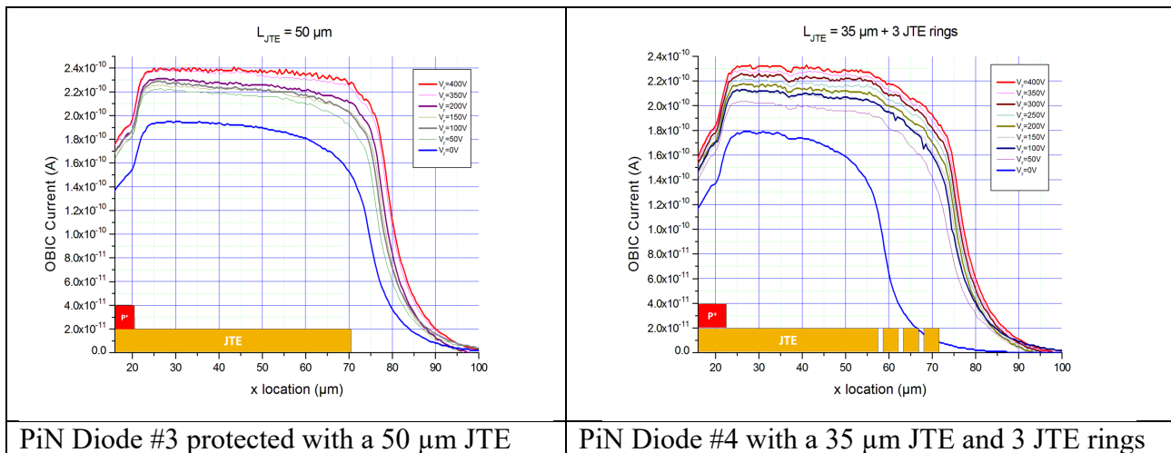
Fig. 6: OBIC measured current versus distance in experiments on 1.7 kV Class PiN diodes with several JTE protections geometries. Basic drawing of each termination is shown as inset.
