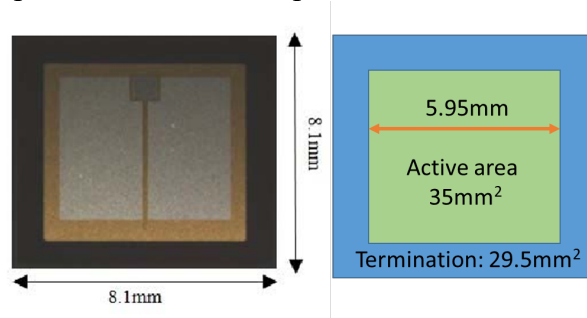
Fig. 1: 6.5kV commercial device picture and evaluation of its respective active and termination area
