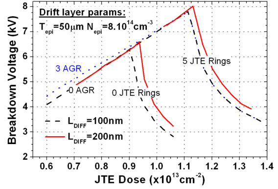
Fig. 3: Schematic of JBS diode termination including (a) JTE with JTE outer rings and P-well FGR (b) comparison of simulated breakdown voltage of a 6.5kV wafer for different JTE + rings designs
