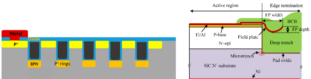
Fig. 4: Schematic of a) a trench rings termination [8] (b) a trench termination filled with Benzocyclobutene BCB [10]
