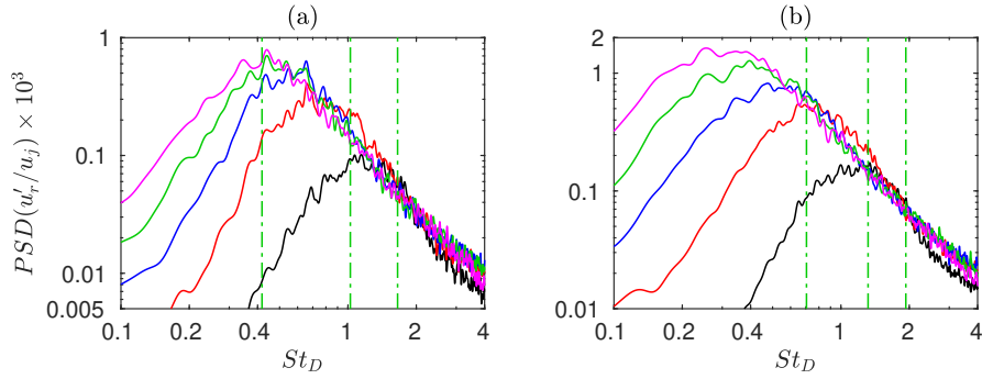
Fig. 13 Power spectral densities of radial velocity fluctuations at r = r_0 for the jet with tripped boundary layers for (a) n_\theta = 0 and (b) n_\theta = 1 as a function of St_D : at — black — z = 2r_0 , — red — z = 4r_0 , — blue — z = 6r_0 , — green — z = 8r_0 and — magenta — z = 10r_0 ; - - - green - - - frequencies of the first three peaks in the pressure spectra at z = 0 and r = 1.5r_0 .
