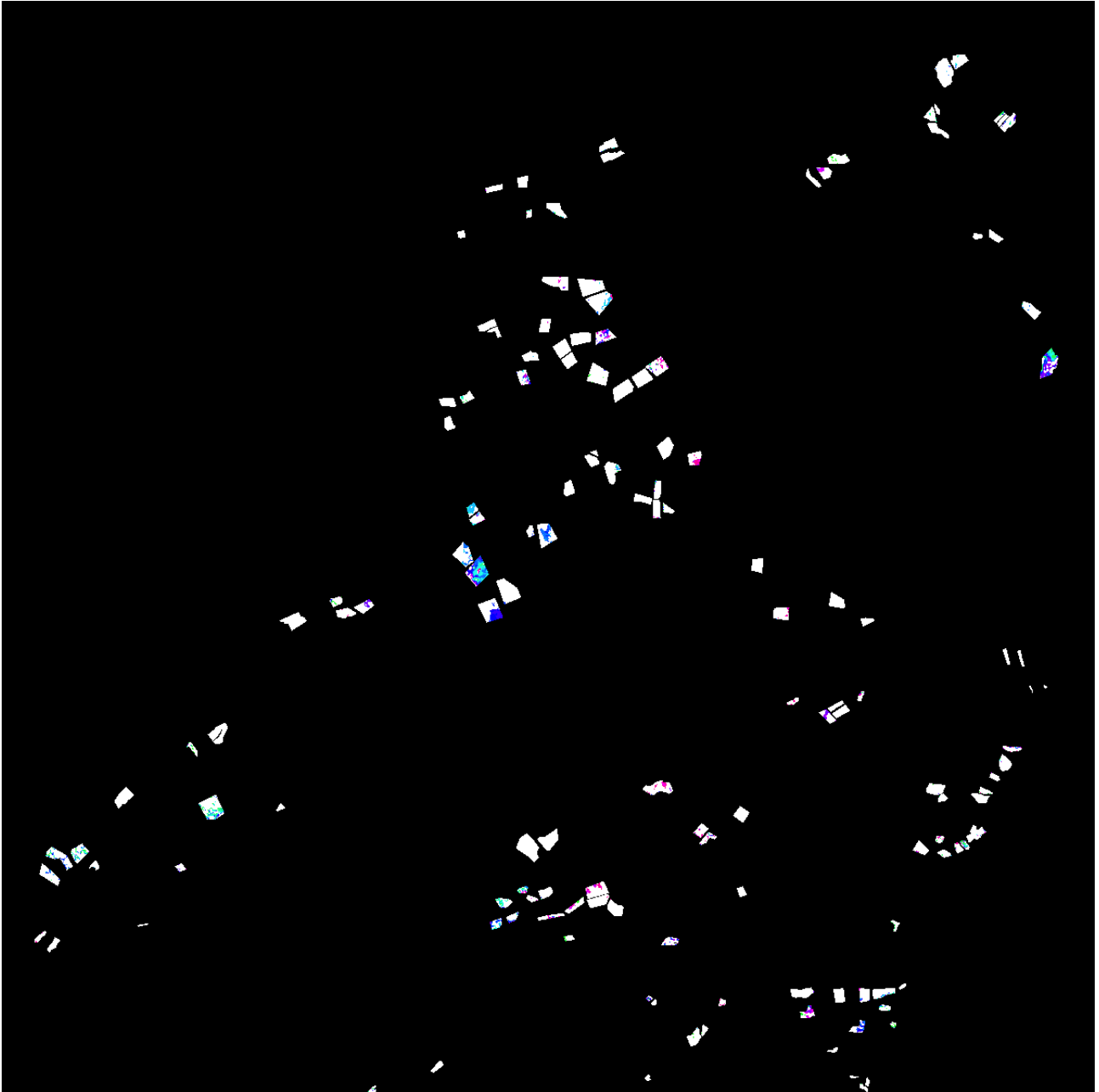
Figure 4. STL-map of the r_2 pattern, for ground truth areas covered by pastures, in the region of la Plaine des Cafres .
