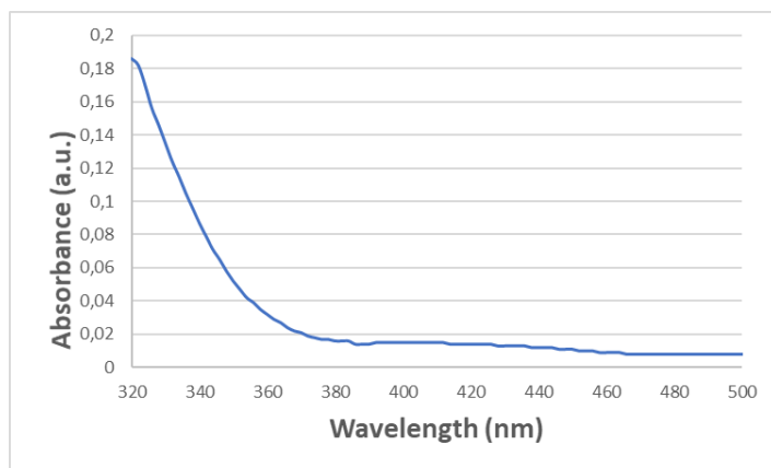
Figure 4: UV-vis spectrum of the Gd_2O_3 nanoparticles suspension.
